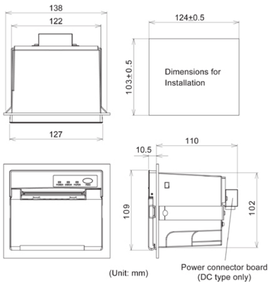
CT-P293 (3 inch model)
