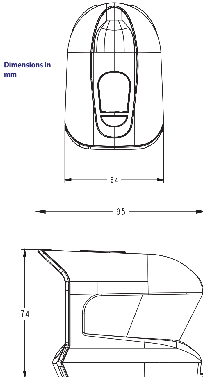
Figure 7. GPS4400 Without Stand
