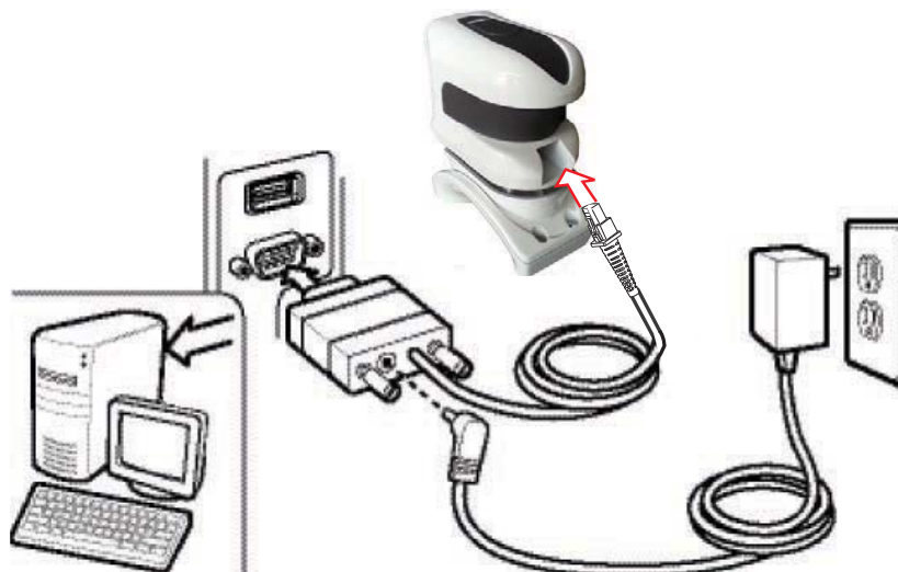
Figure 1. RS-232 Connection
