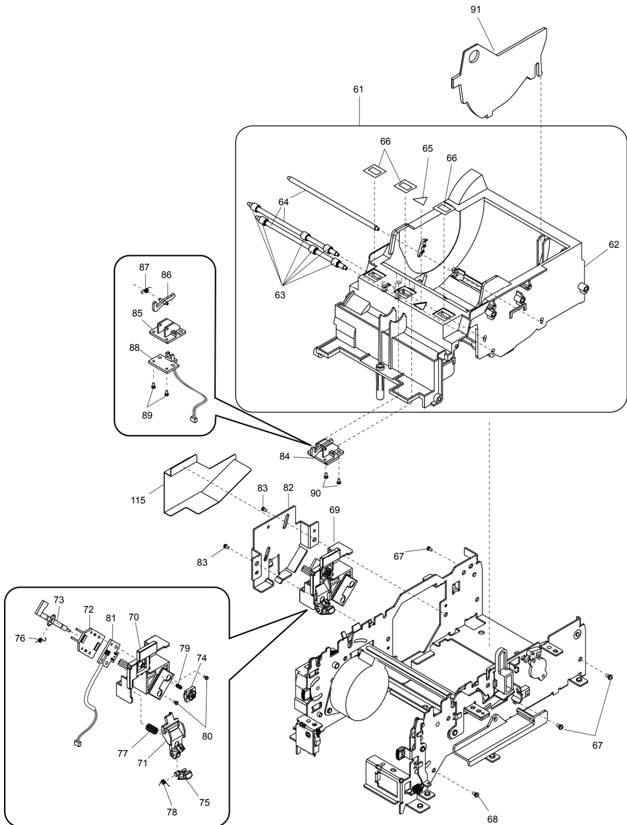
Exploded diagram 5
