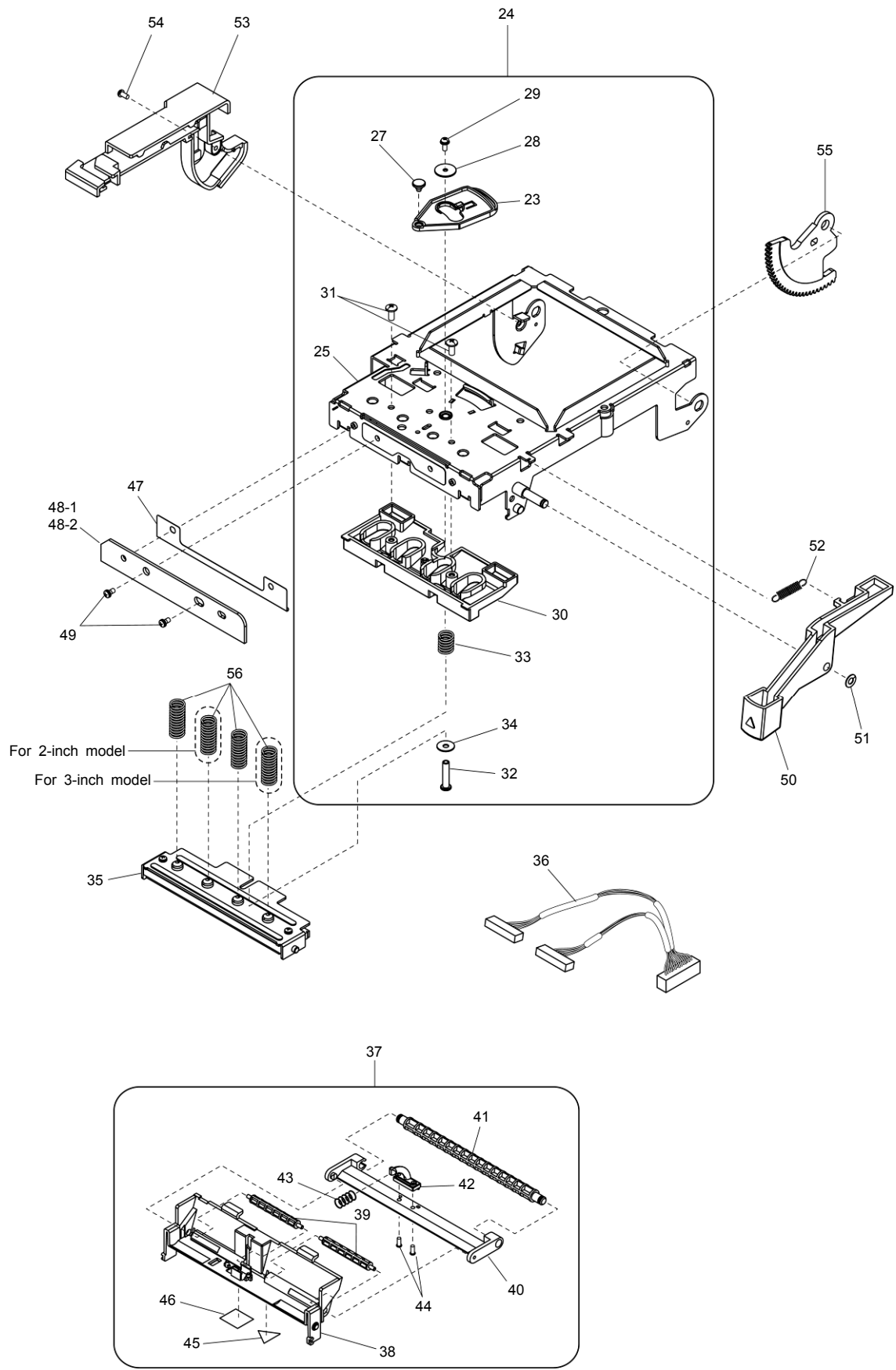
Exploded diagram 4
