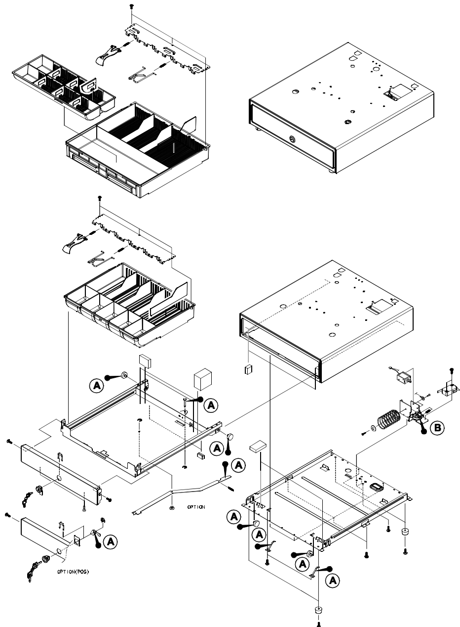
Figure 6-10 Lubrication Points of the G-Drawer(4B8C,5B6C)
