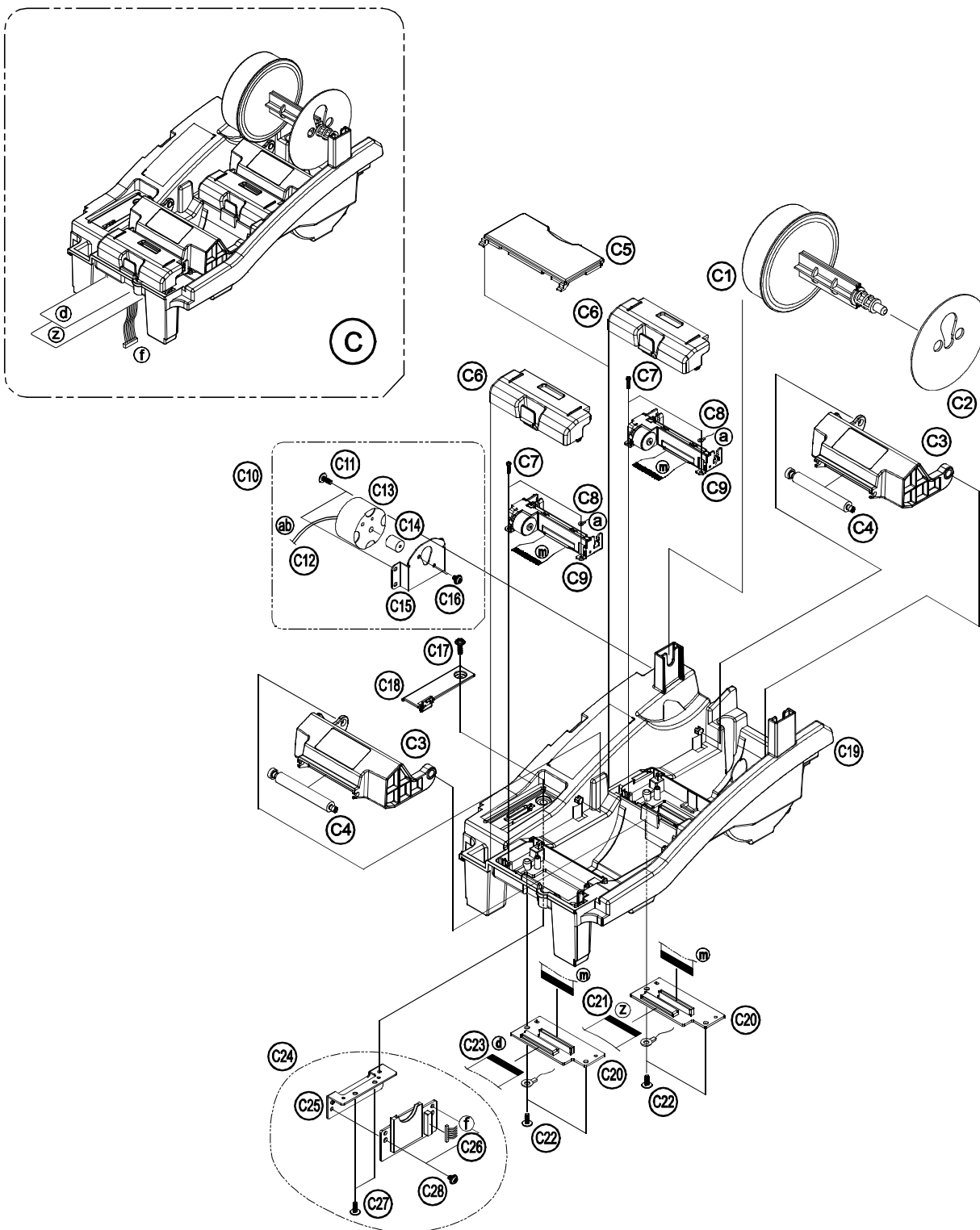
Figure 6-5 ASS'Y PRINTER
