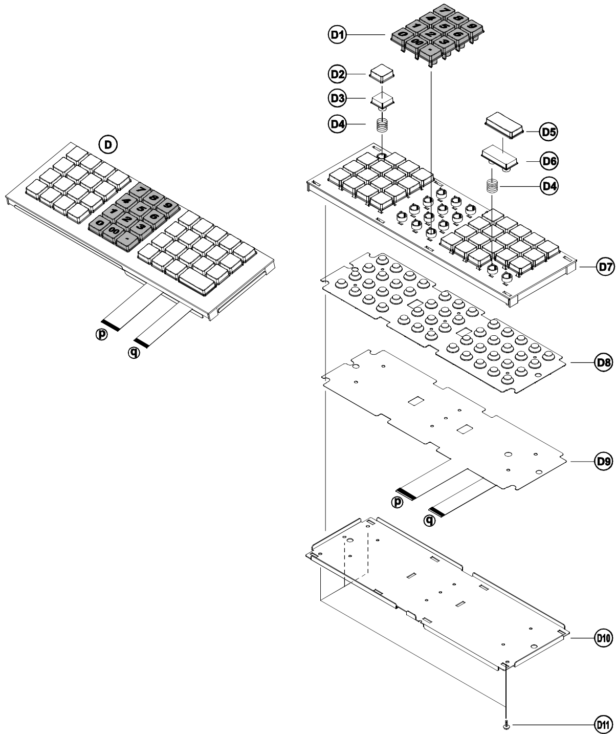
Figure 6-6 ASS'Y-KEYBOARD (48 Key)
