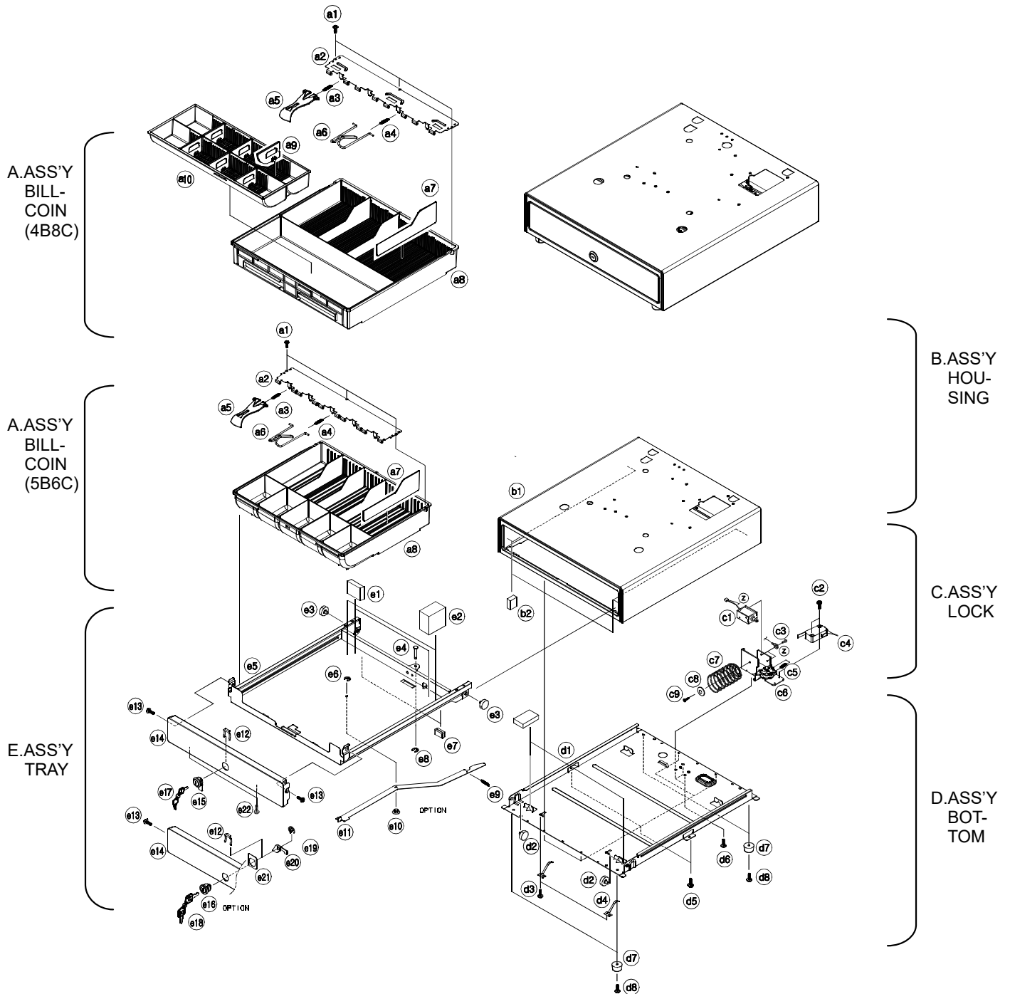
Figure 6-9 ASS'Y-DRAWER (G-DRAWER:4B8C,5B6C)
