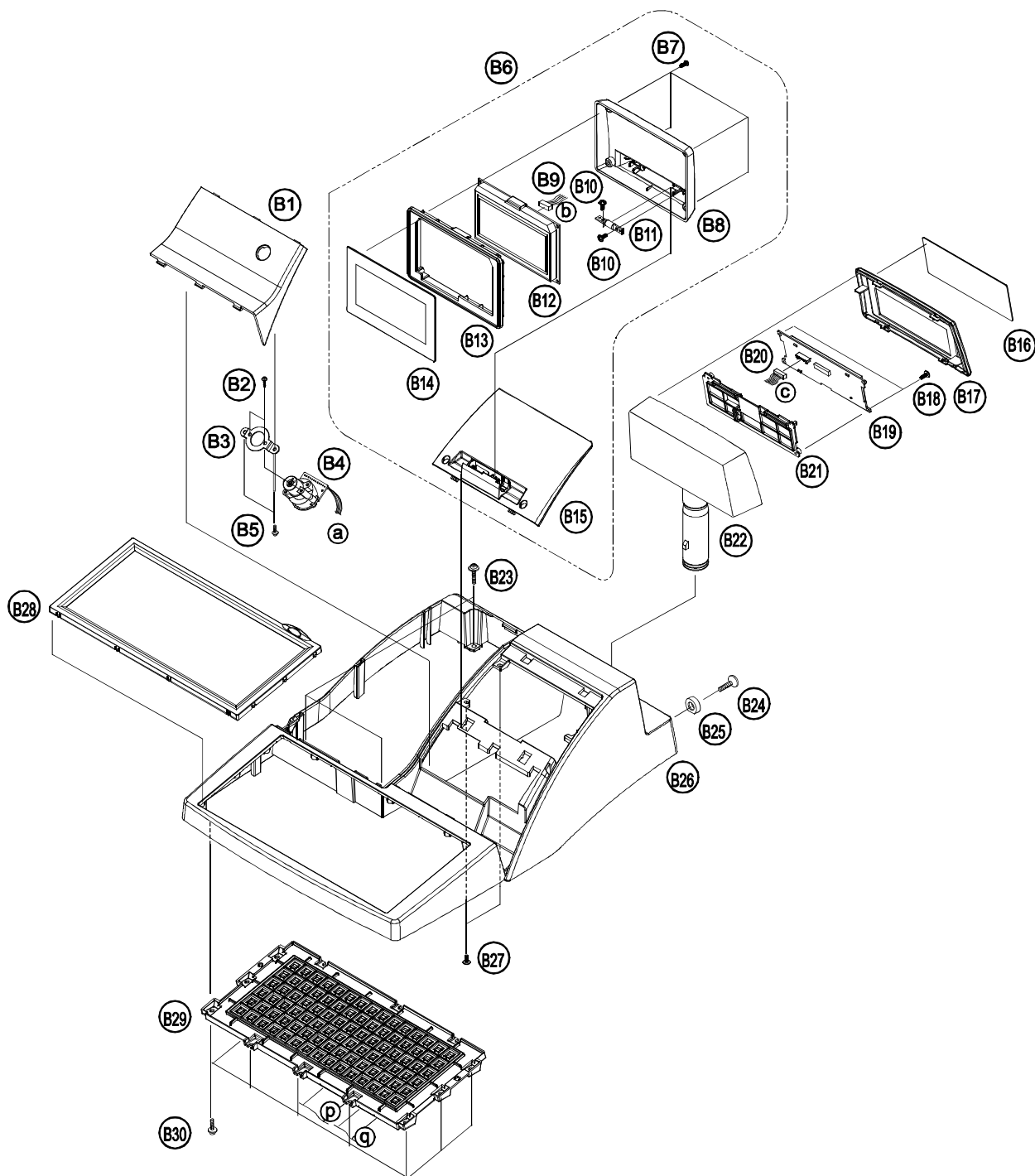
Figure 6-4 ASS'Y CASE-UPPER(NR-500)
