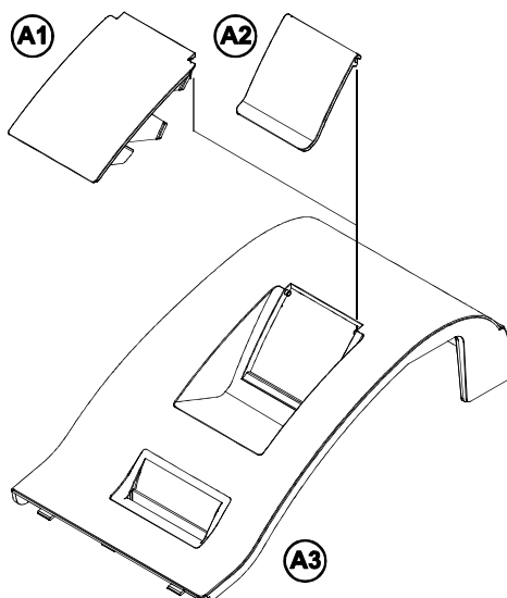
Figure 6-2 ASS'Y COVER-PRINTER
