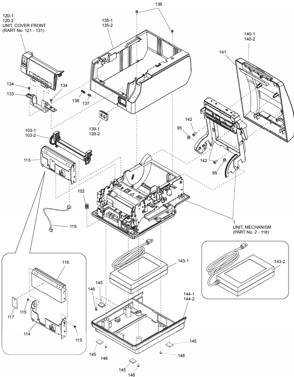
Exploded diagram 1
