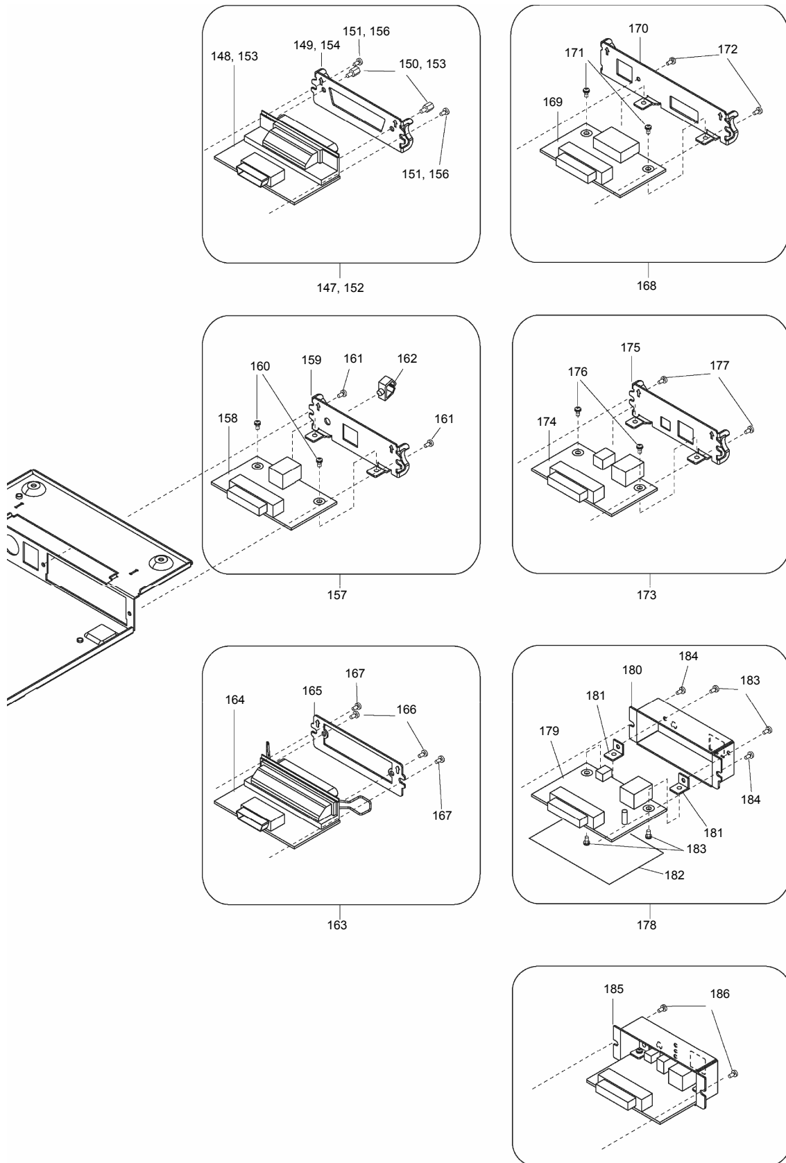
Exploded diagram 7
