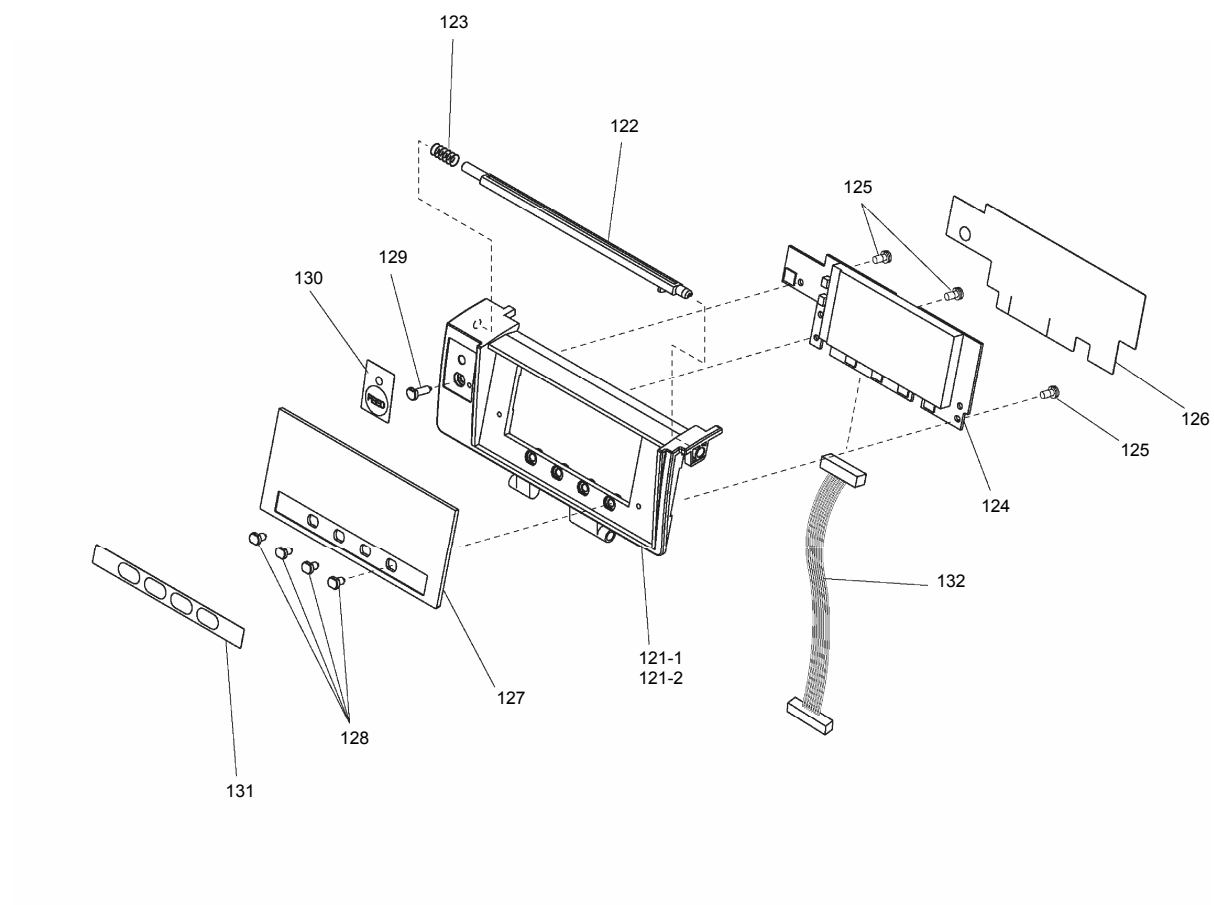
Exploded diagram 2
