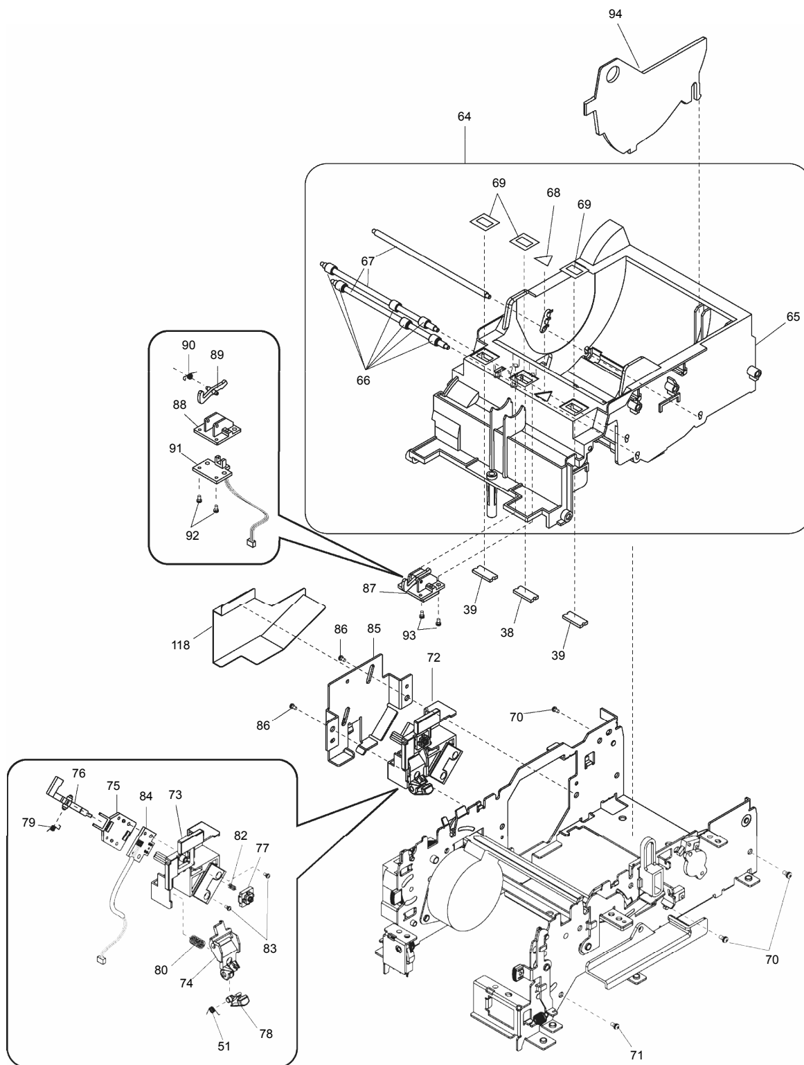
Exploded diagram 5
