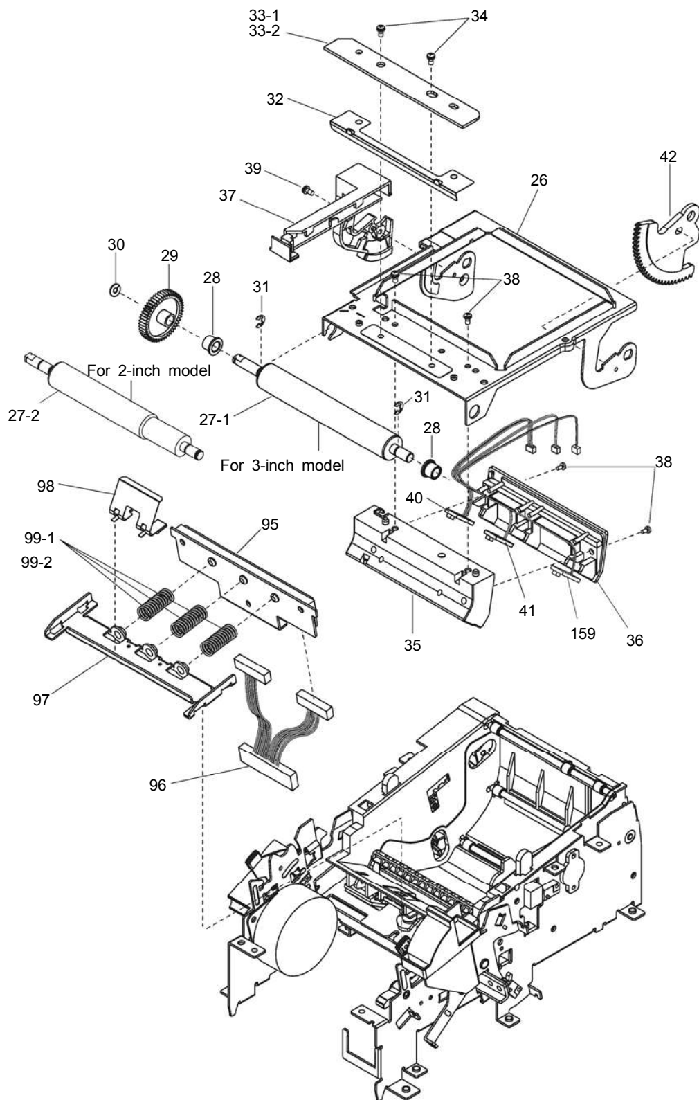
Exploded diagram 4
