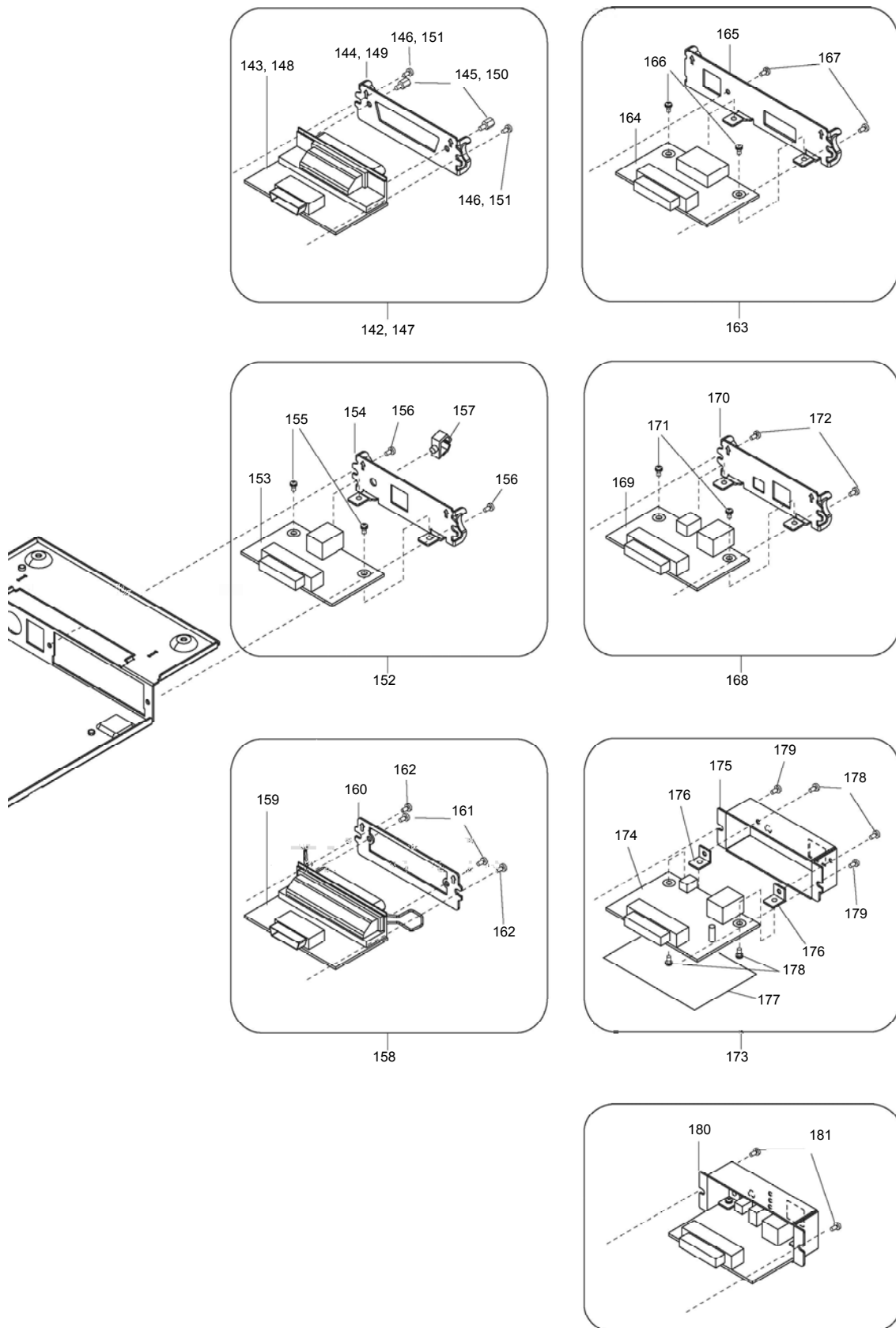
Exploded diagram 7
