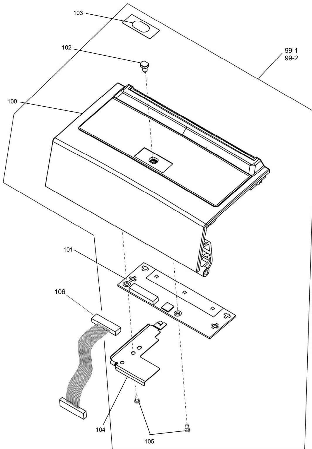
Exploded diagram 2
