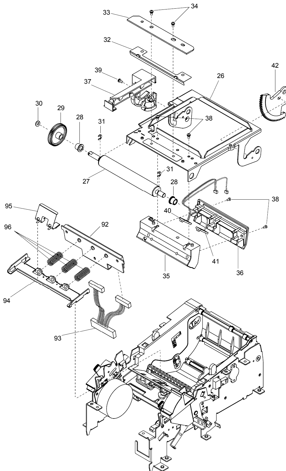
Exploded diagram 4
