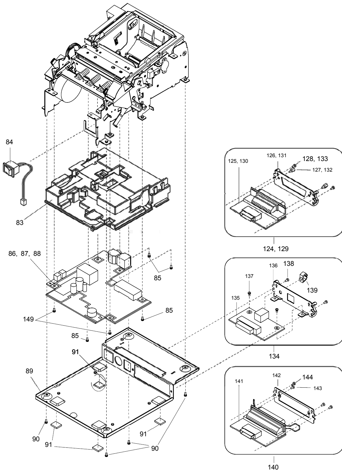
Exploded diagram 3
