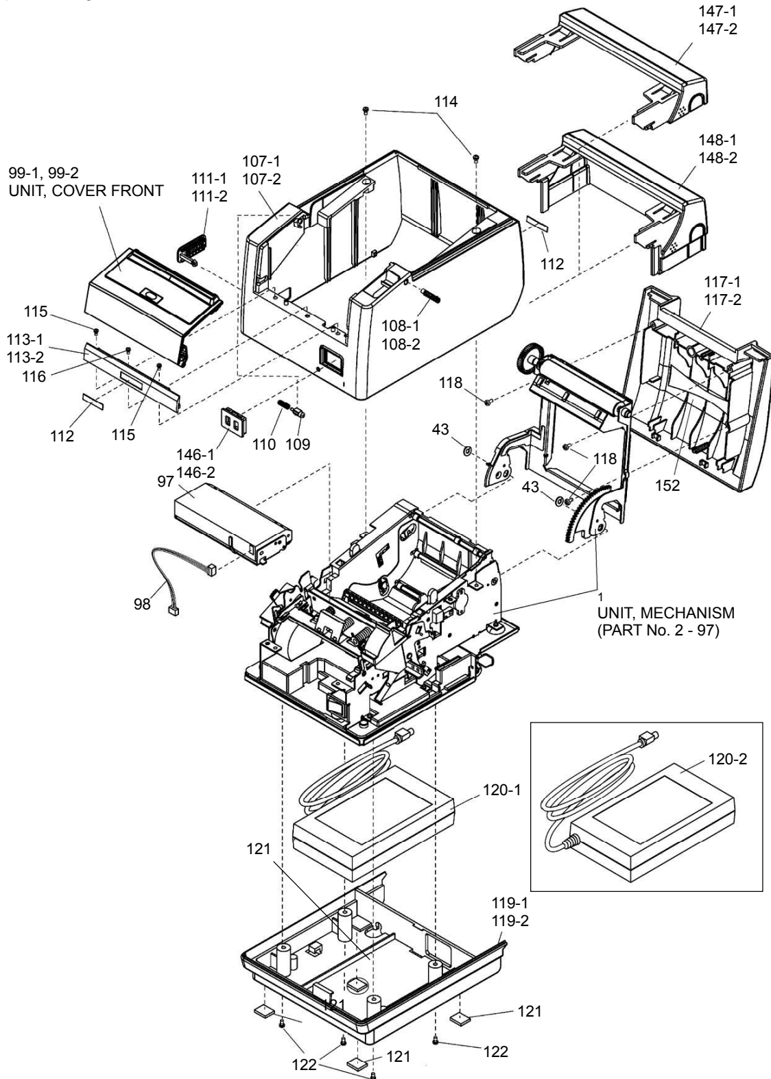
Exploded diagram 1
