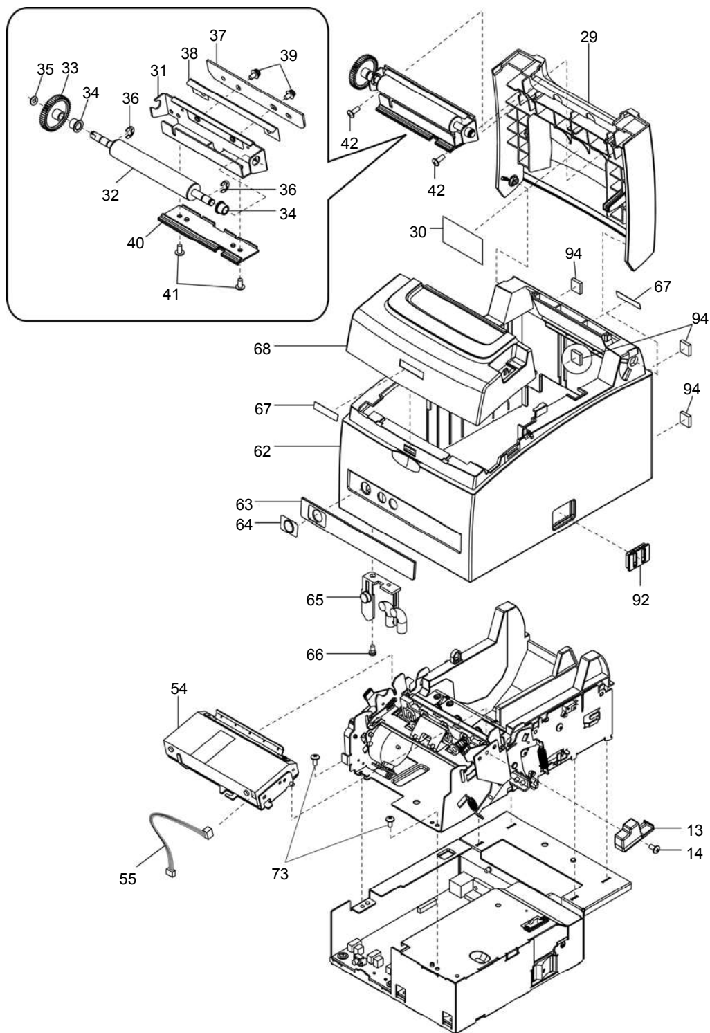
Exploded diagram 1
