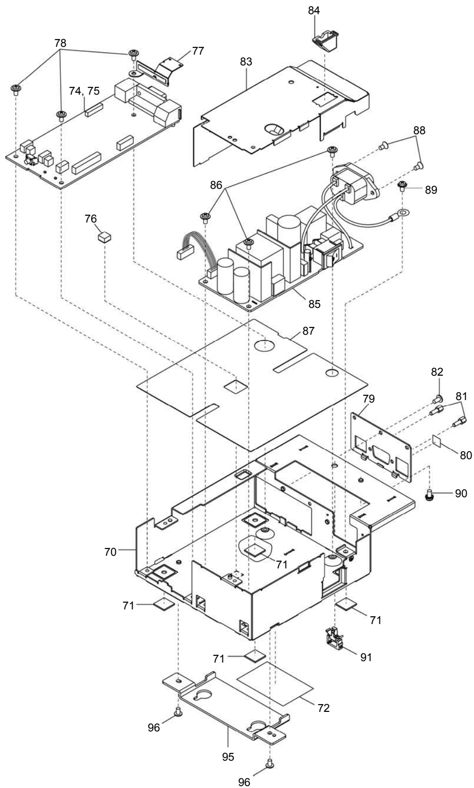
Exploded diagram 4
