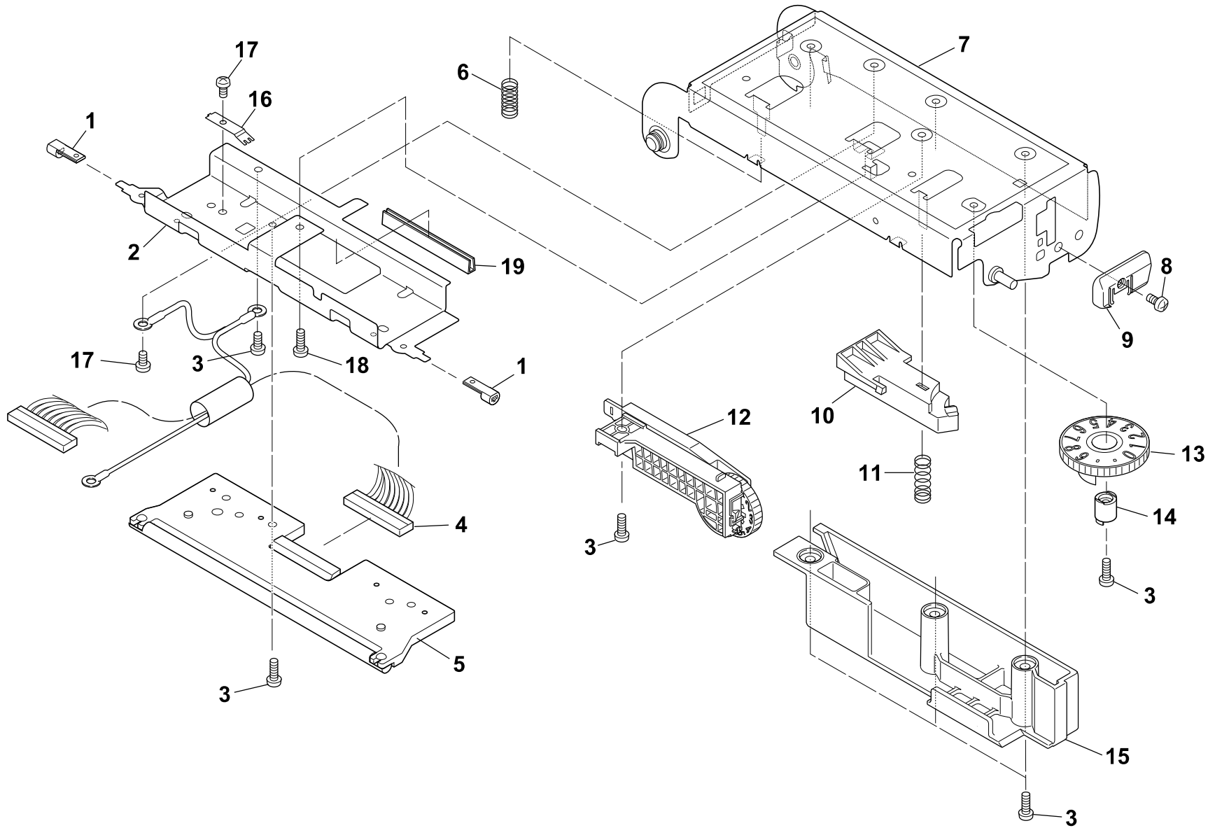
DRAWING NO. 4 Unit, Head-DT (Rev. 0)
