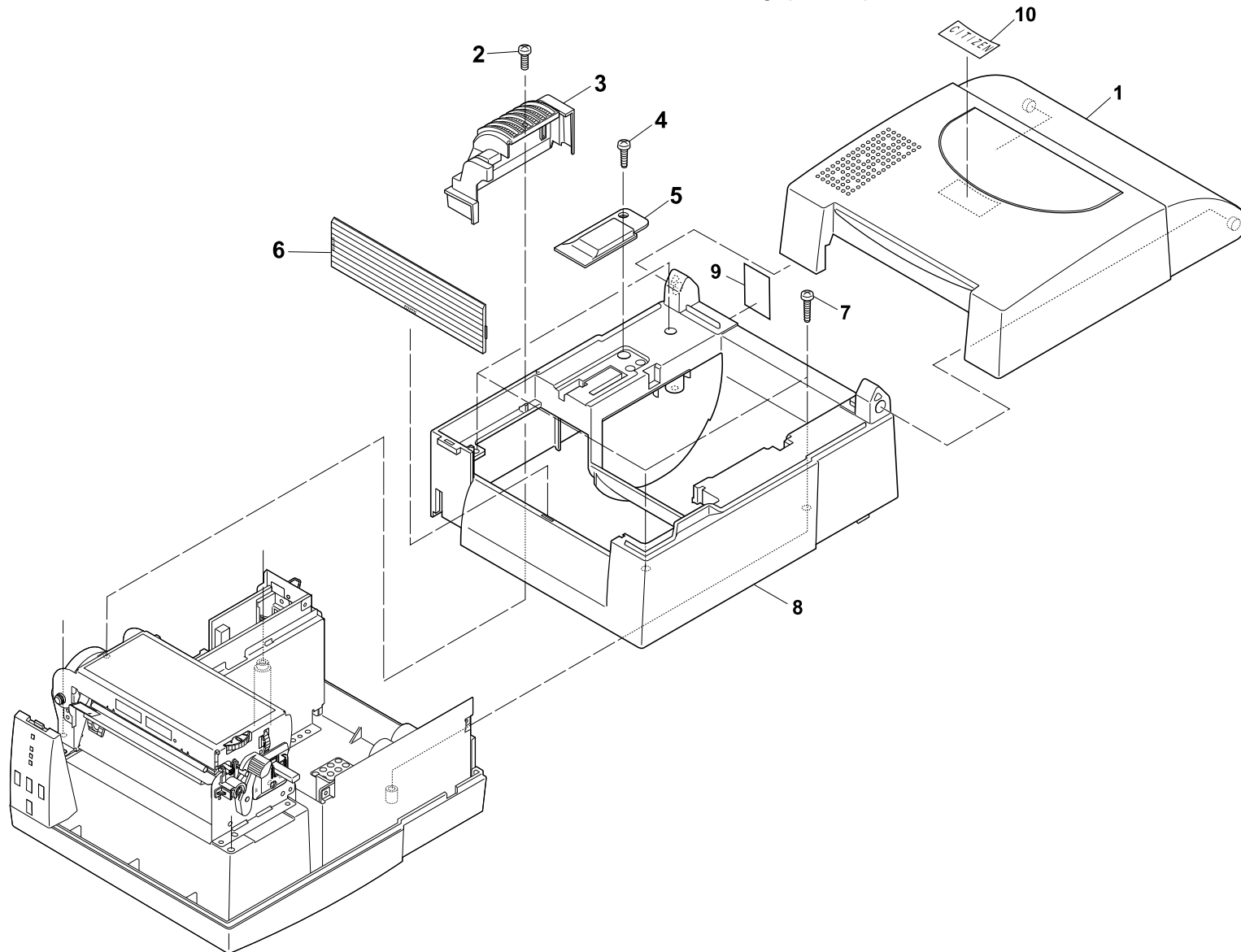
DRAWING NO. 1 General Assembly (Rev. 0)
