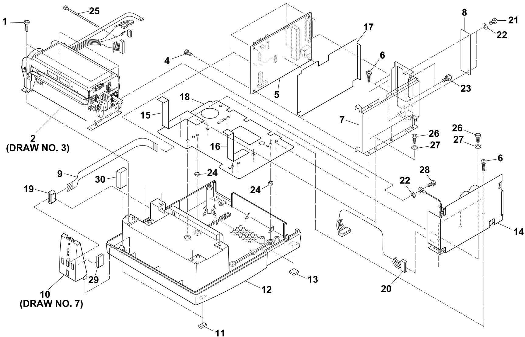
DRAWING NO. 2 Base Unit (Rev. 0)
