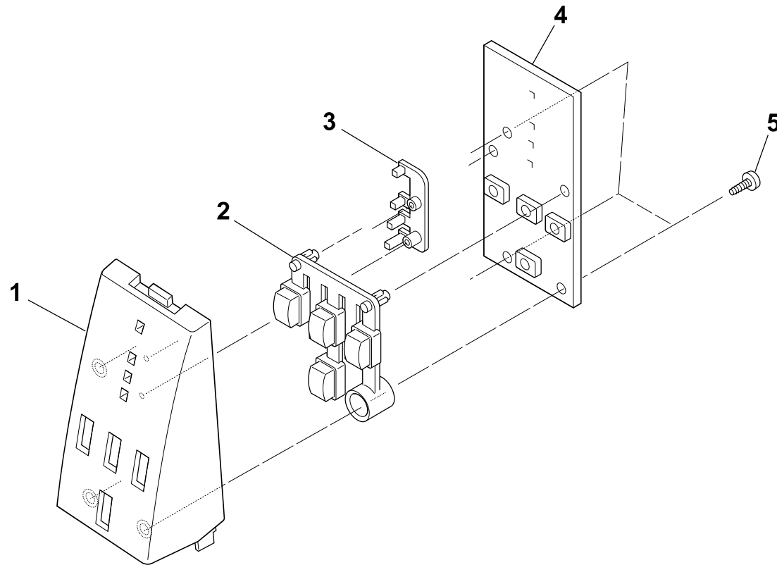
DRAWING NO. 7 Unit, Control Panel (Rev. 0)
