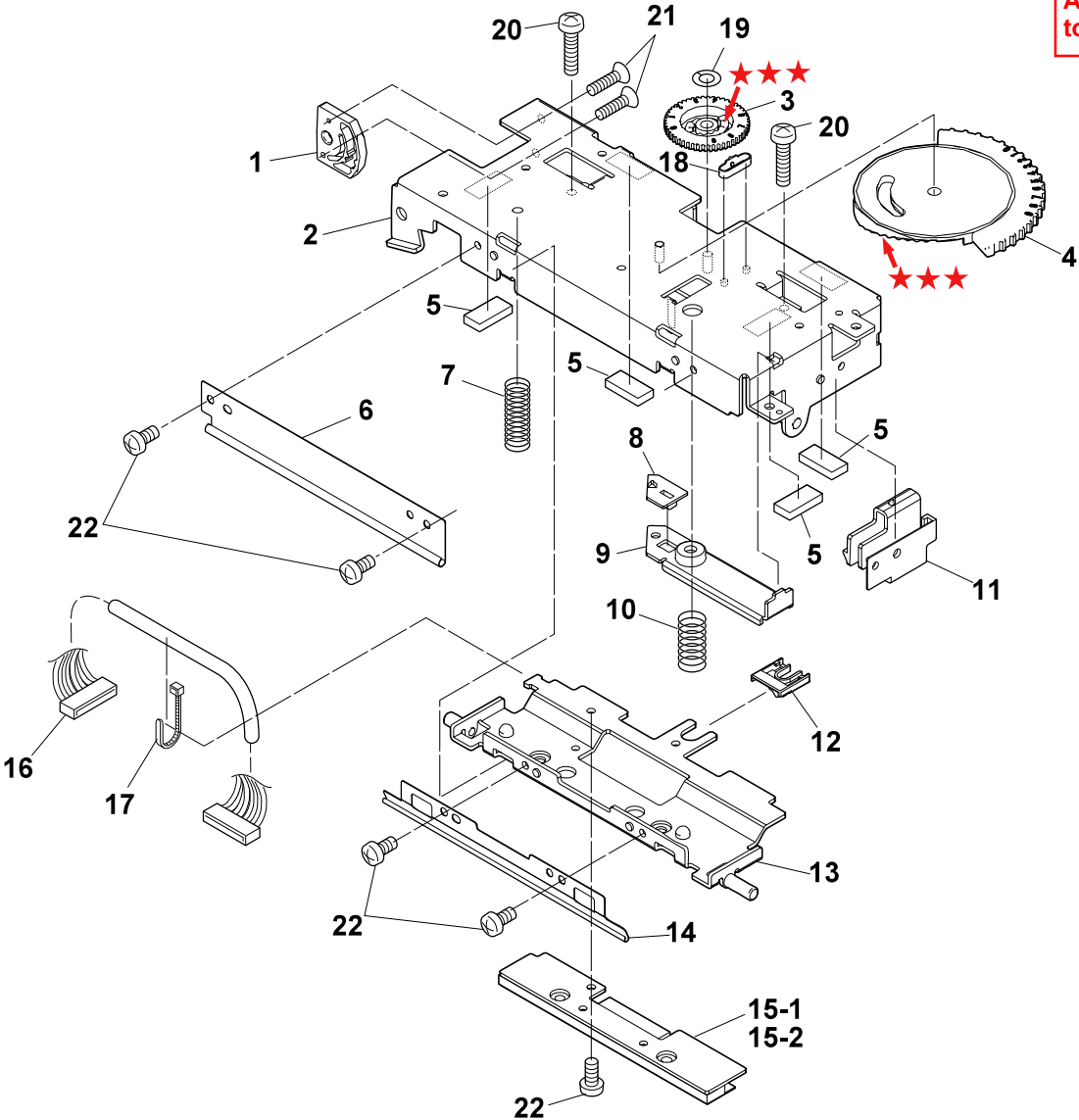
DRAWING NO. 4 SA2 Cover Frame (Rev. 0)
