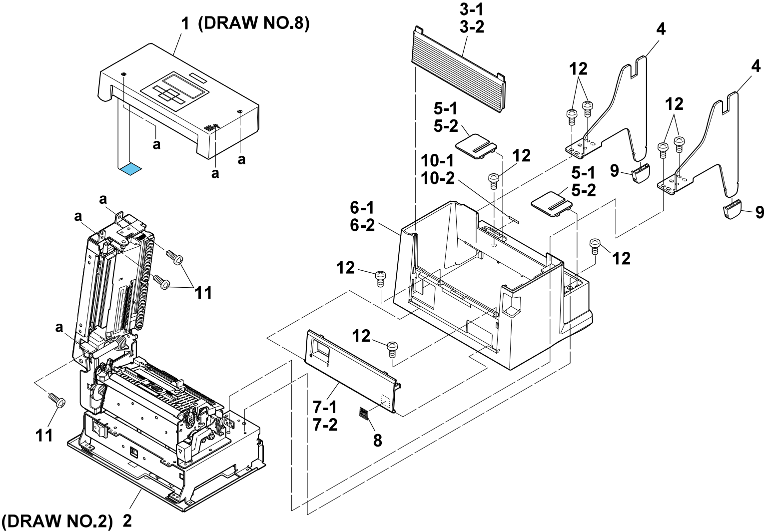
DRAWING NO. 1 General Assembly (Rev. 0)
