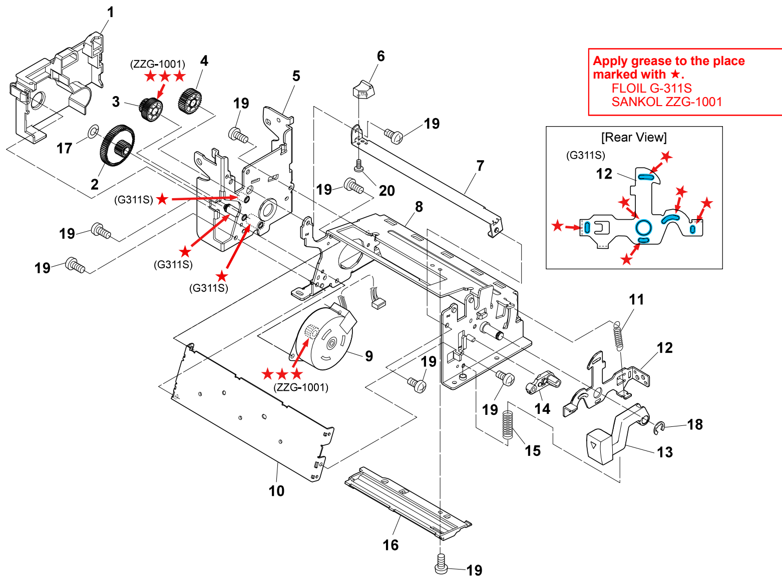
DRAWING NO. 7 SA2 Main Frame (Rev. 0)
