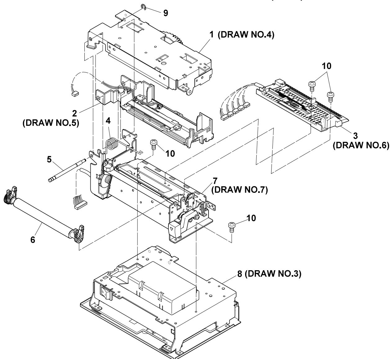
DRAWING NO. 2 SA Mechanism (Rev. 0)
