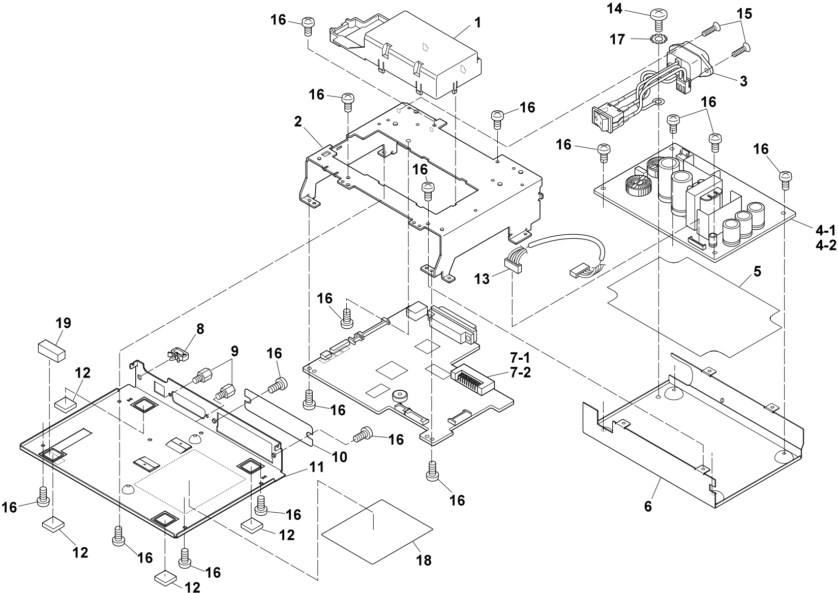
DRAWING NO. 3 SA2 Base Frame (Rev. 0)
