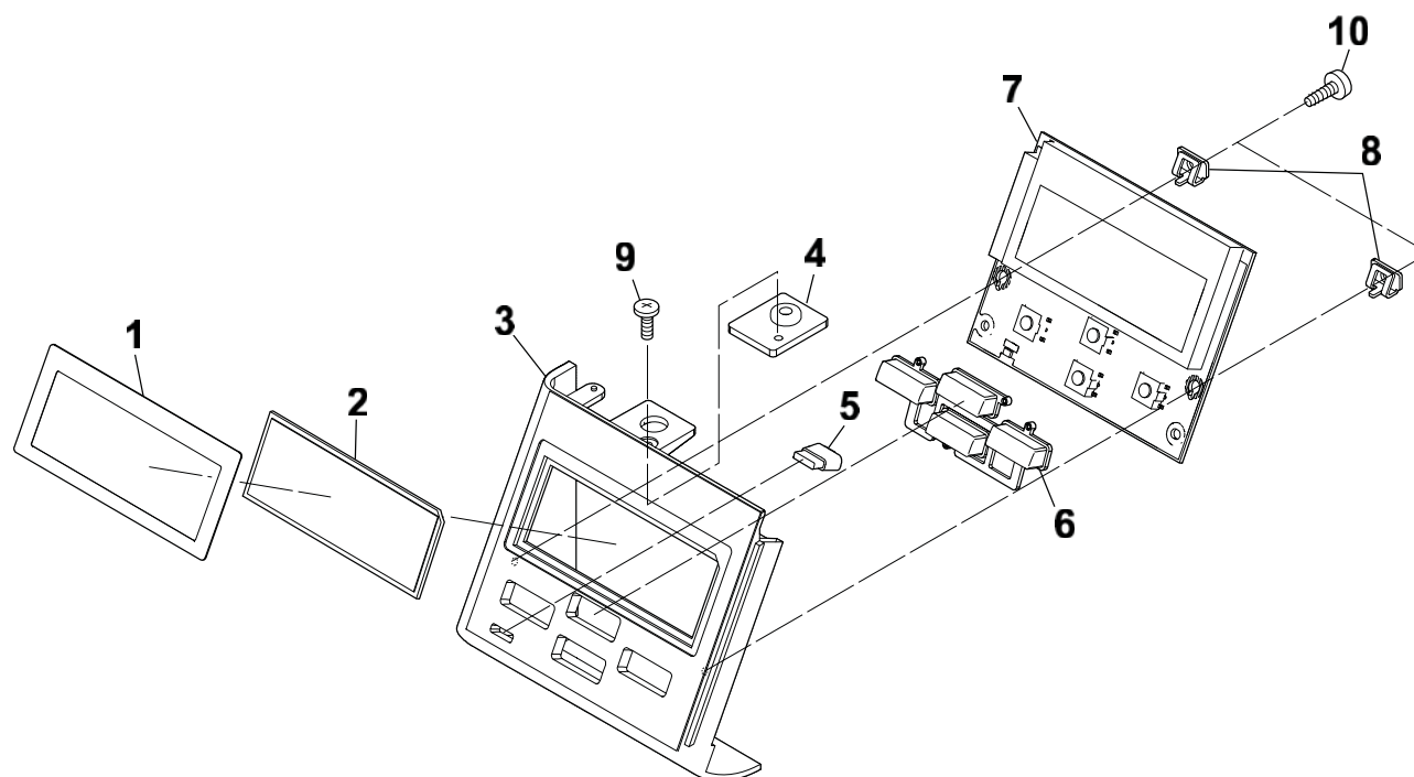
DRAWING NO. 7 Unit Opepane (Rev. 0)
