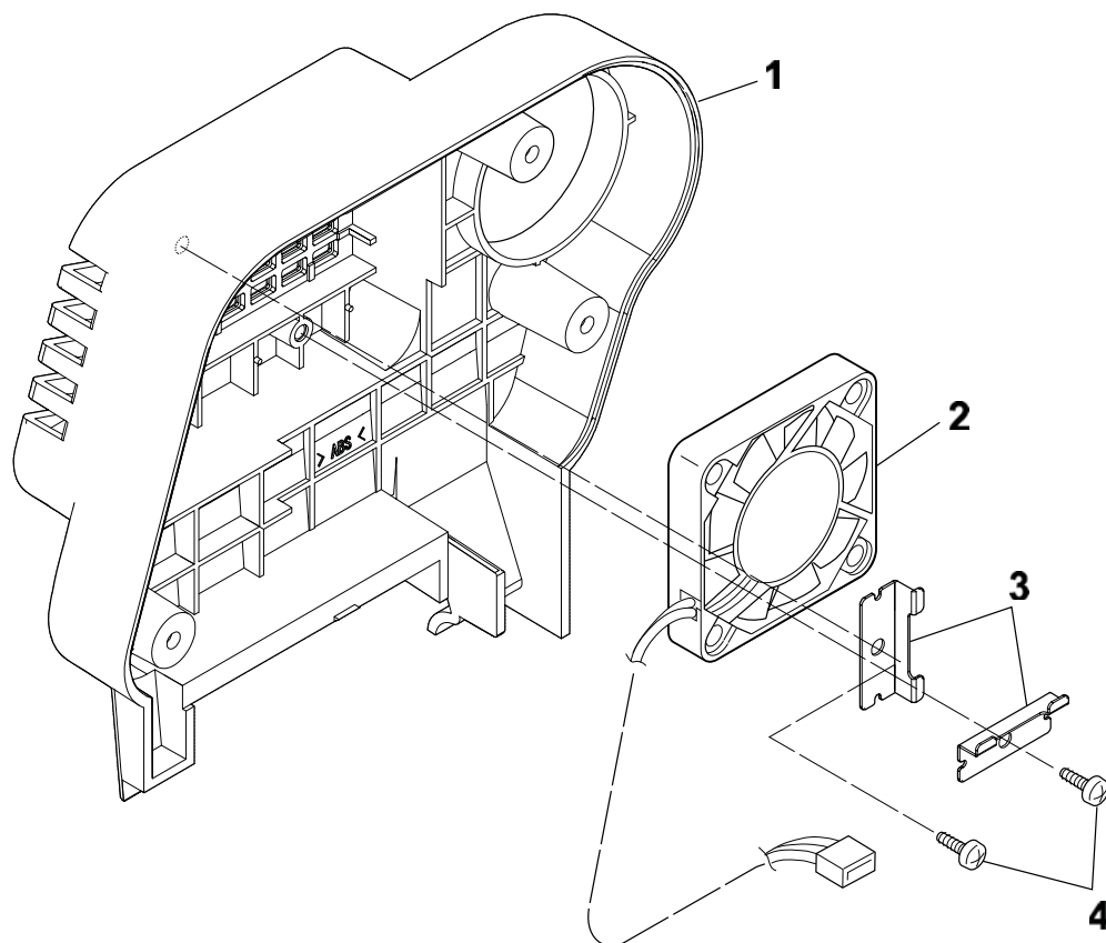
DRAWING NO. 9 SA2 Ribbon Unit Fan (Rev. 0)
