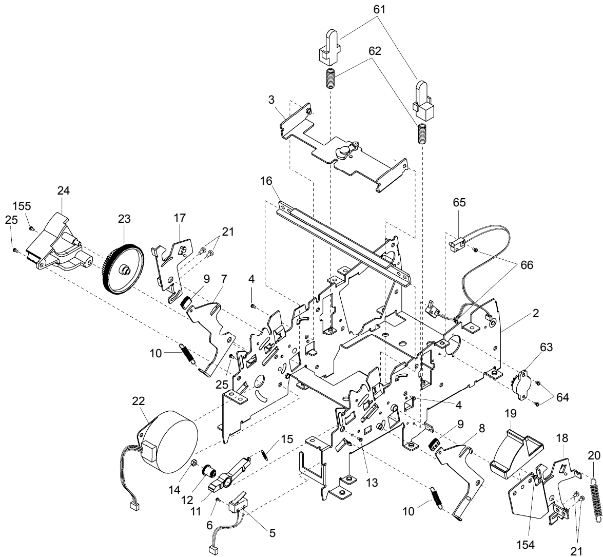
Exploded diagram 6
