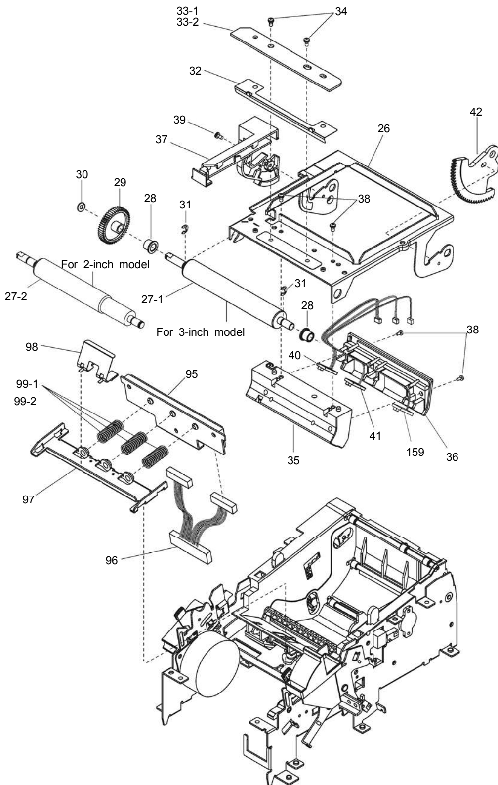
Exploded diagram 4
