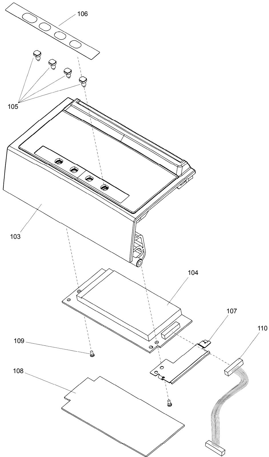
Exploded diagram 2
