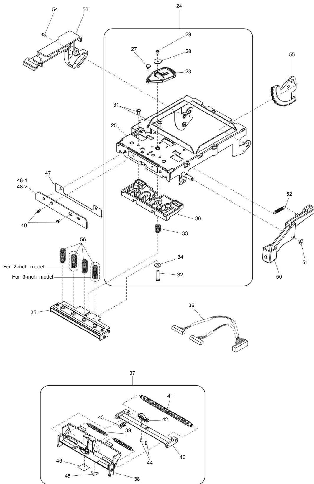
Exploded diagram 4
