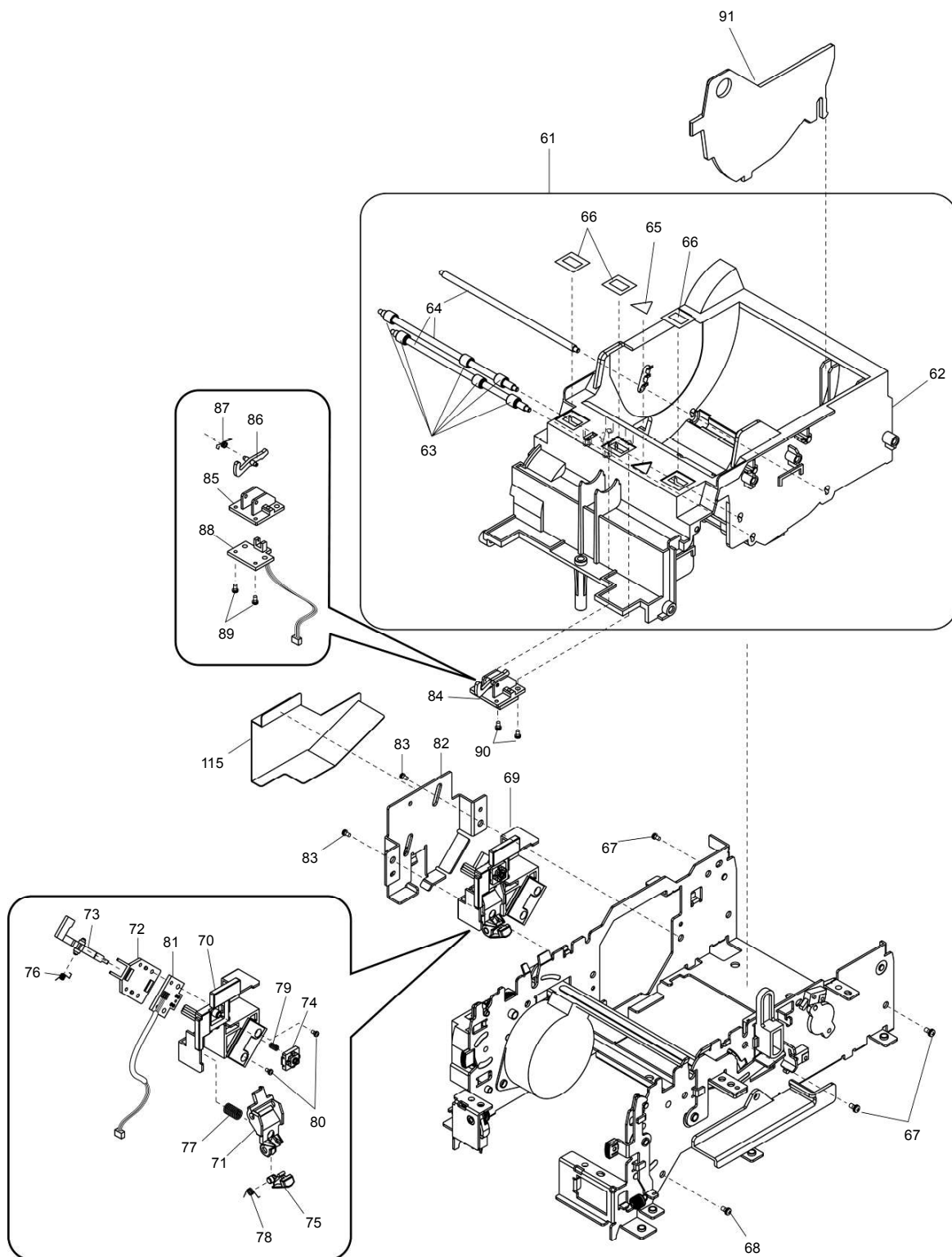
Exploded diagram 5
