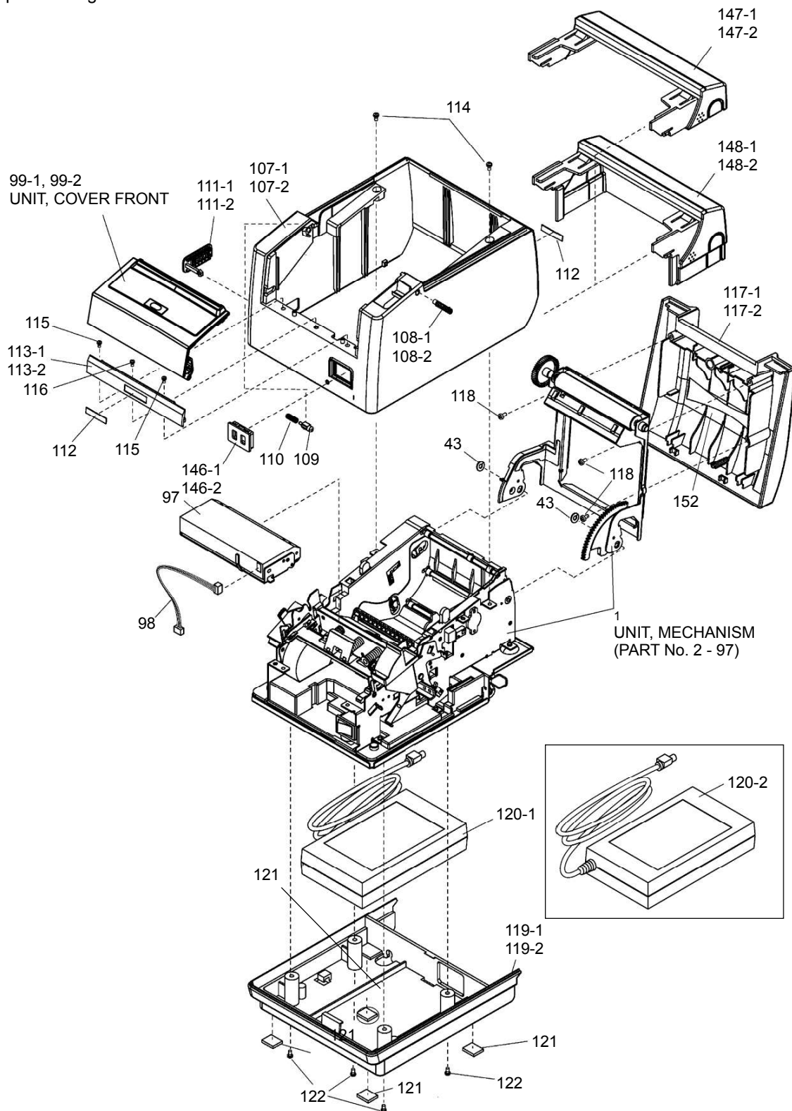
Exploded diagram 1
