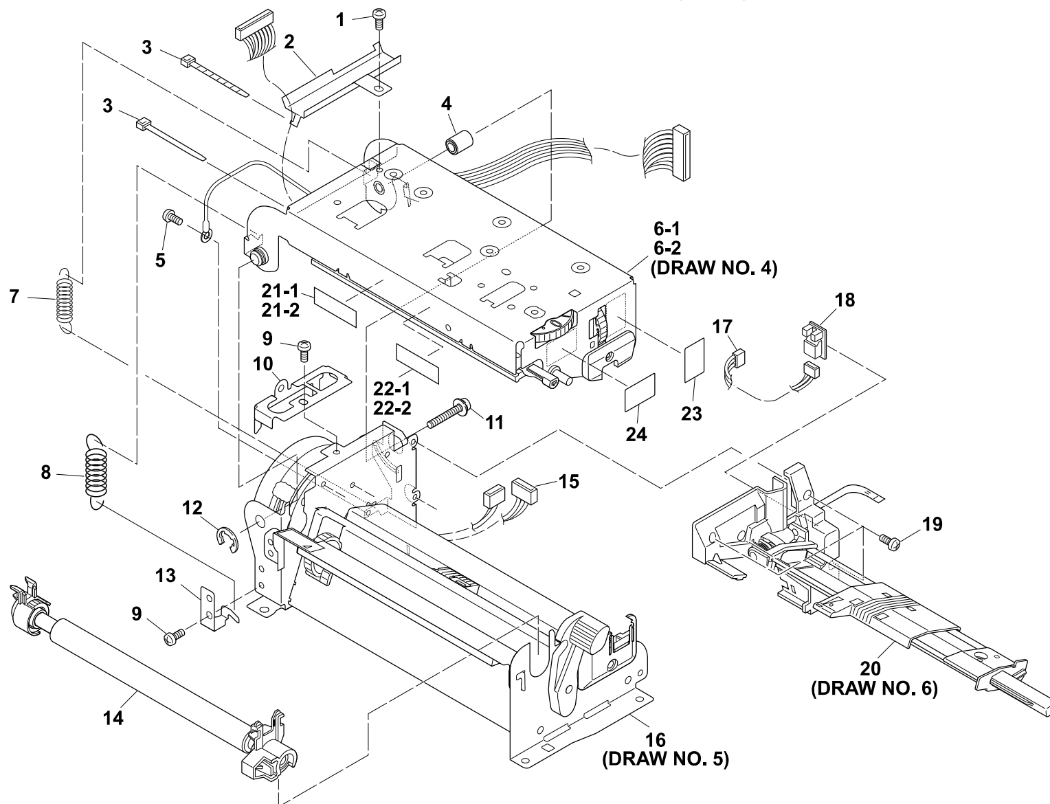
DRAWING NO. 3 Unit, Mechanism (Rev. 0)
