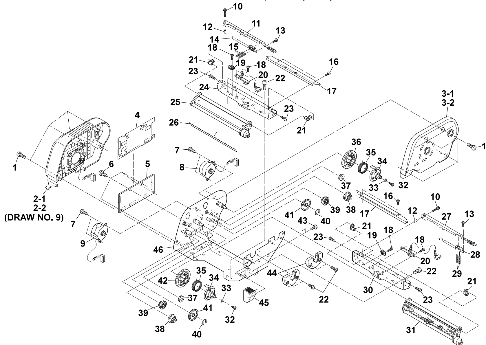
DRAWING NO. 8 Unit, Ribbon (Rev. 0)
