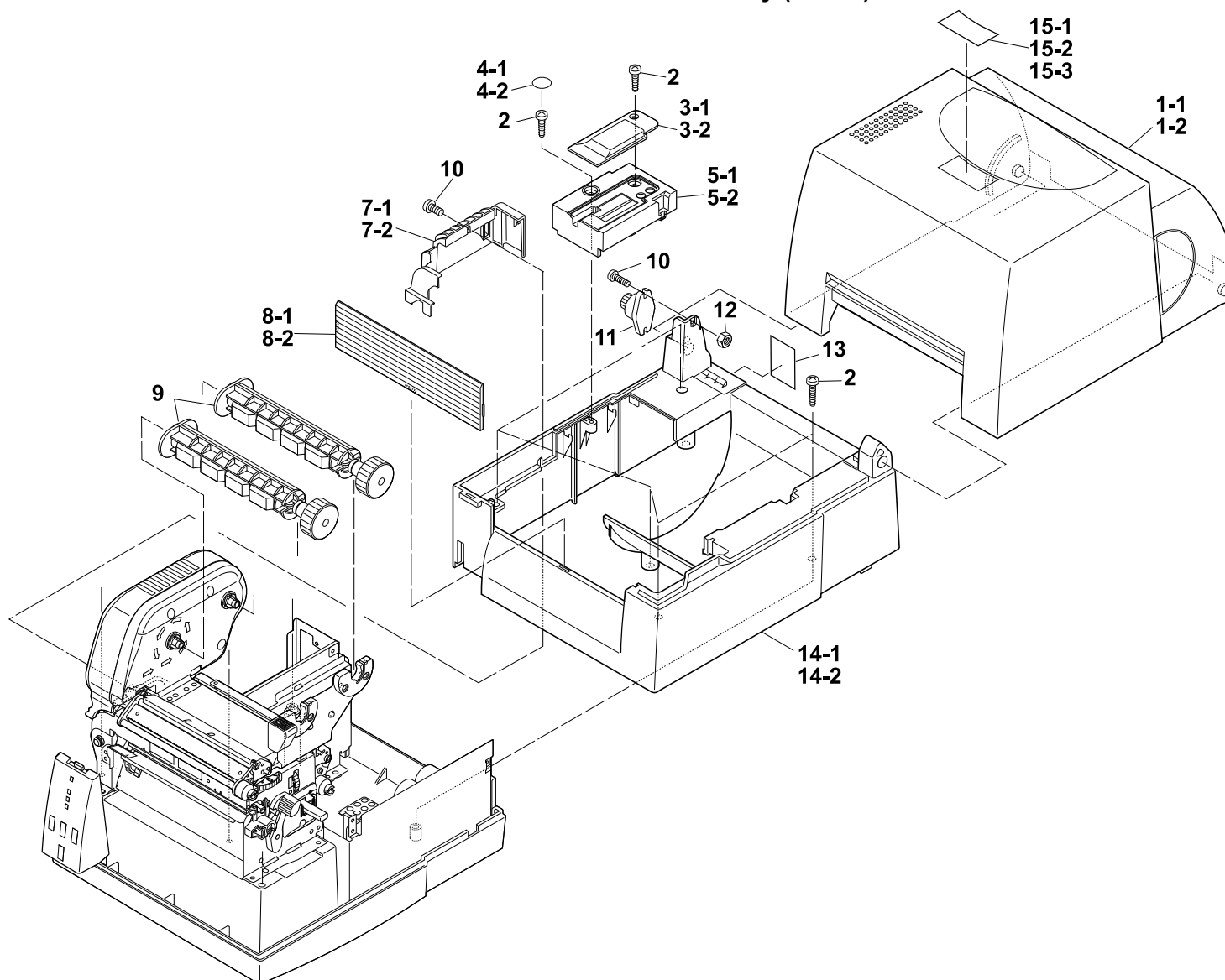
DRAWING NO. 1 General Assembly (Rev. 0)
