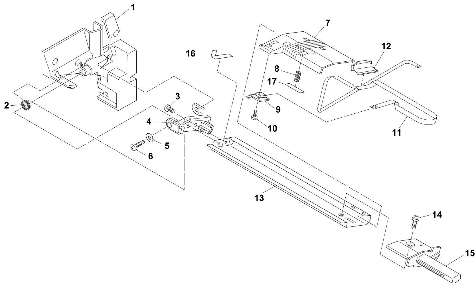
DRAWING NO. 6 Unit, Sensor U (Rev. 0)
