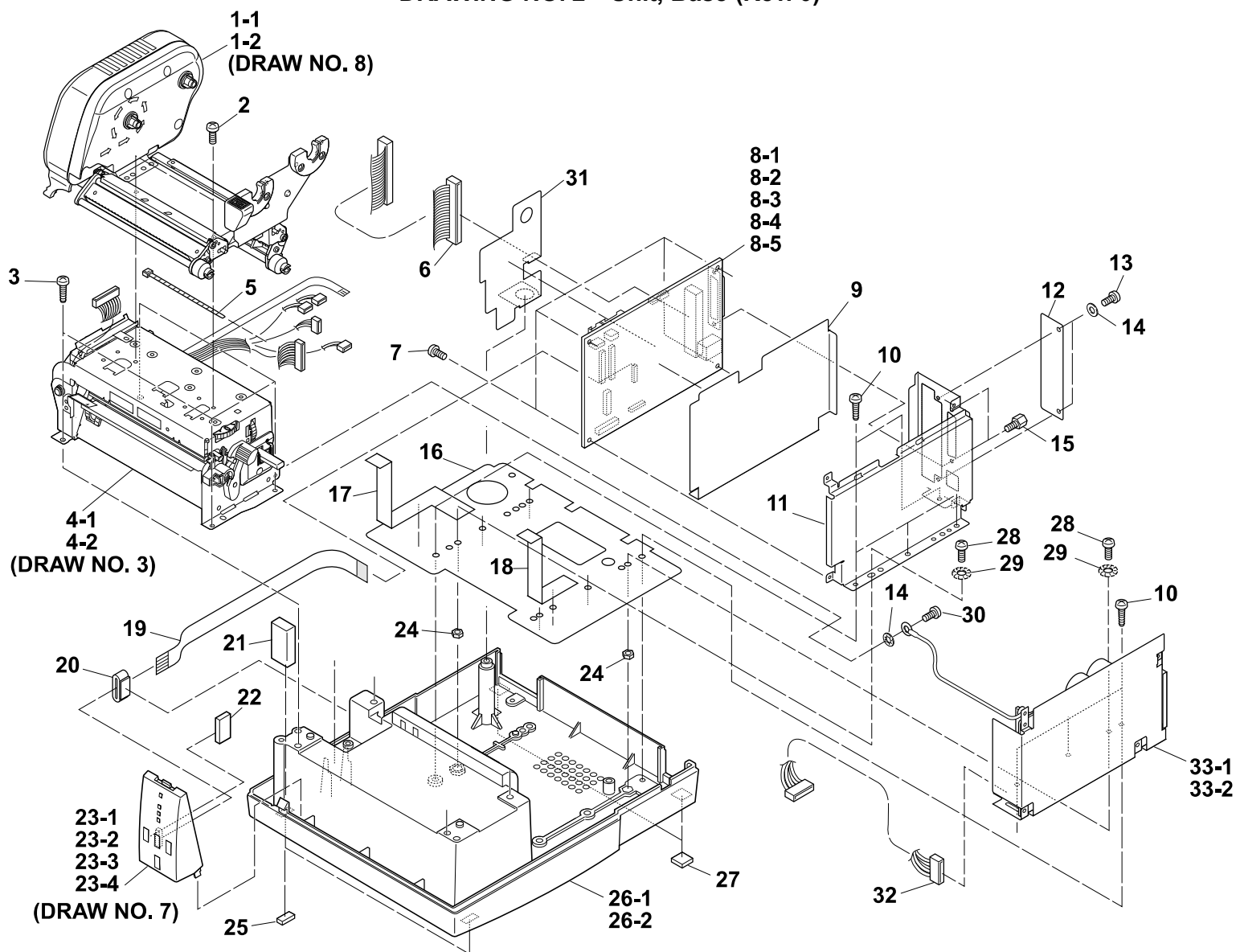
DRAWING NO. 2 Unit, Base (Rev. 0)
