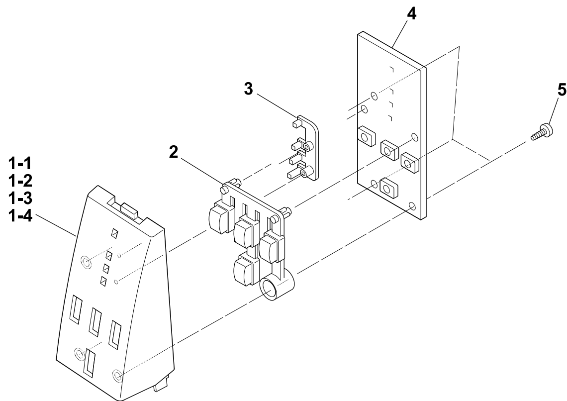
DRAWING NO. 7 Unit, Control Panel (Rev. 0)
