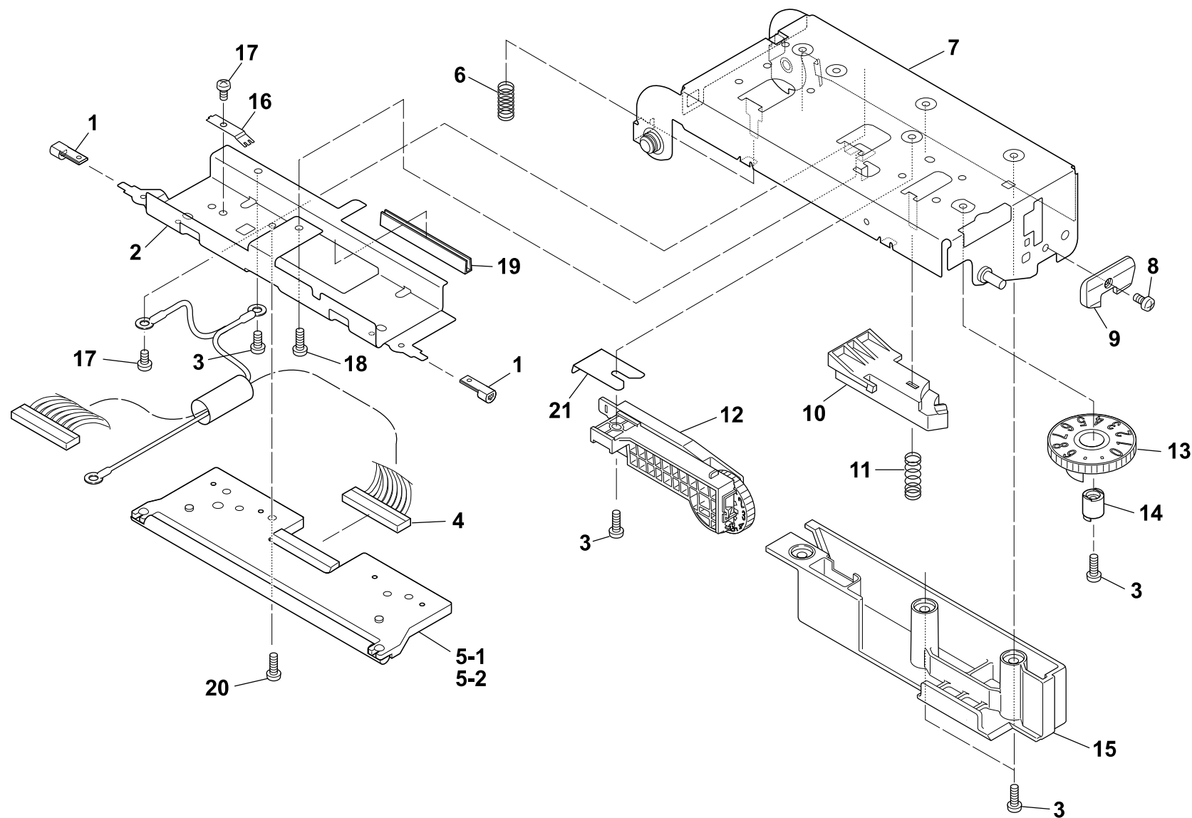
DRAWING NO. 4 Unit, Head-TT (Rev. 0)
