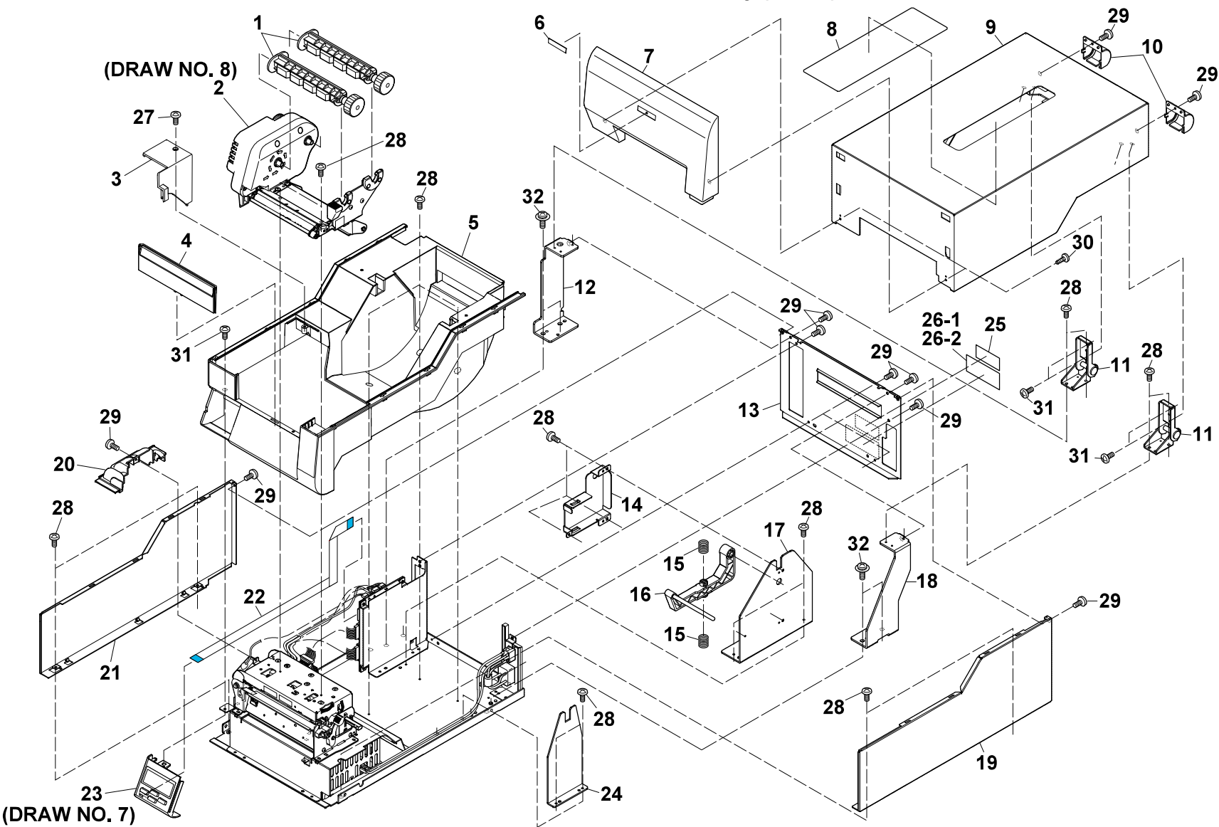
DRAWING NO. 1 General Assembly (Rev. 1)
