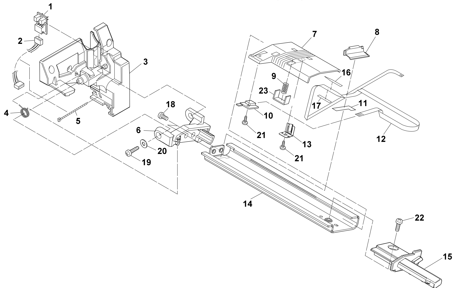
DRAWING NO. 6 Unit Sensor U (Rev. 0)
