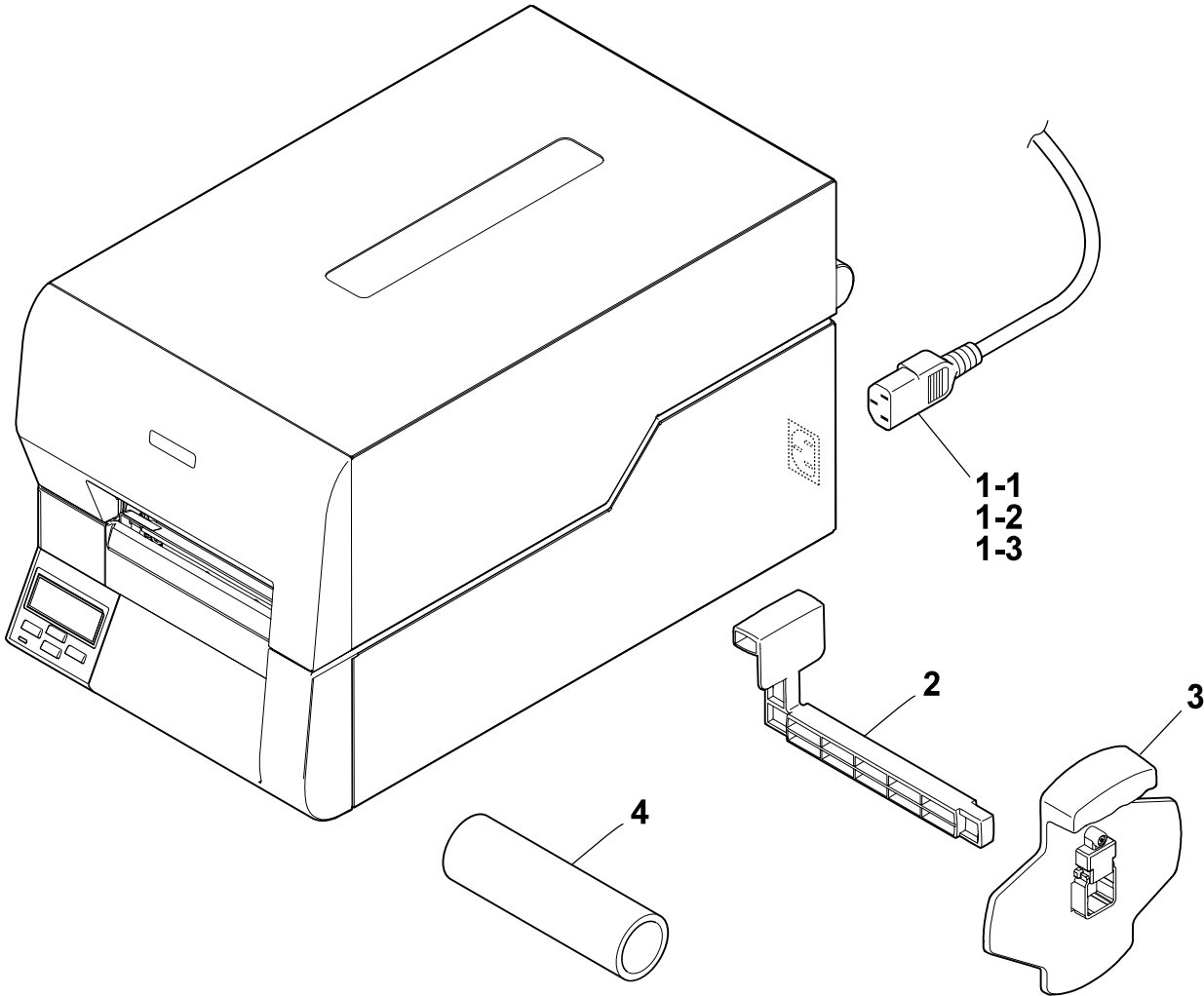
DRAWING NO. 10 Accessories (Rev. 0)
