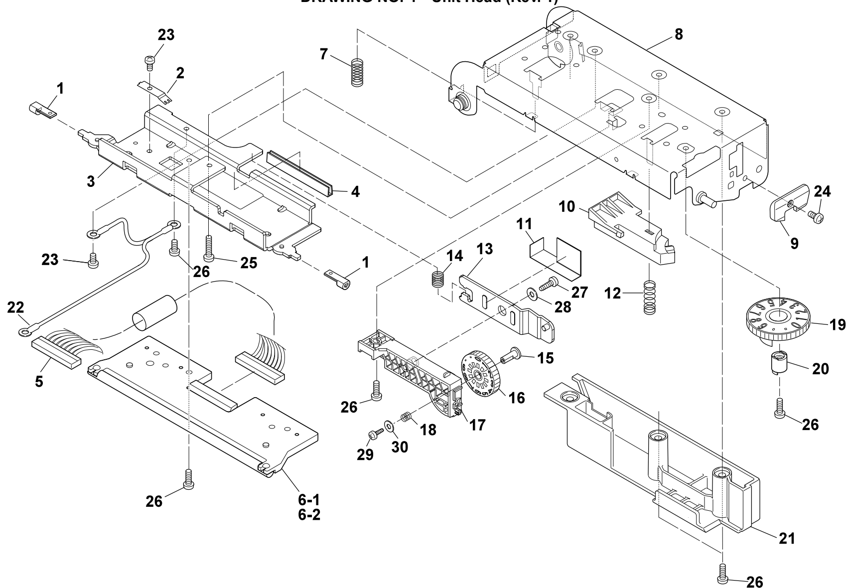
DRAWING NO. 4 Unit Head (Rev. 1)
