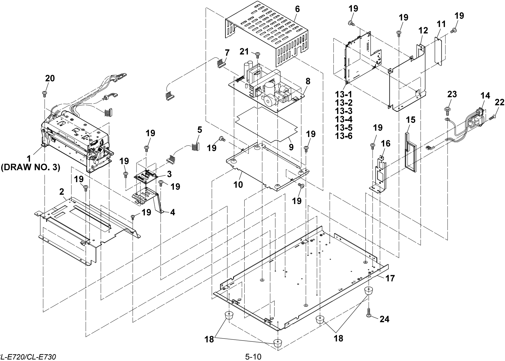
DRAWING NO. 2 Unit Base (Rev. 1)
