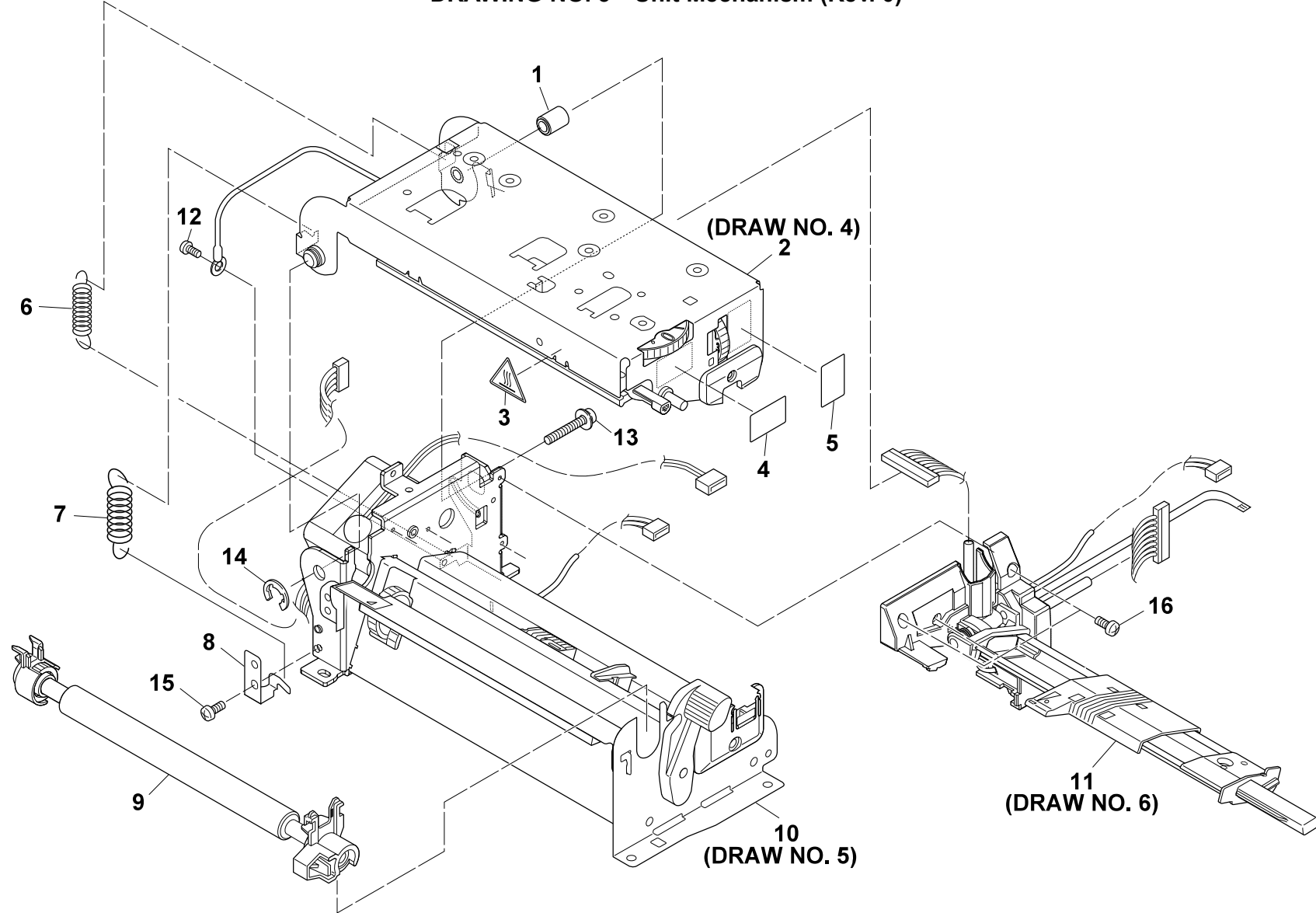
DRAWING NO. 3 Unit Mechanism (Rev. 0)
