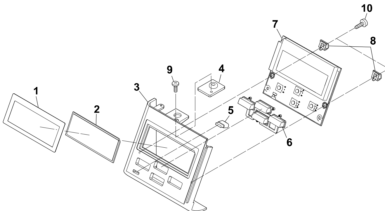
DRAWING NO. 7 Unit Opepane (Rev. 0)
