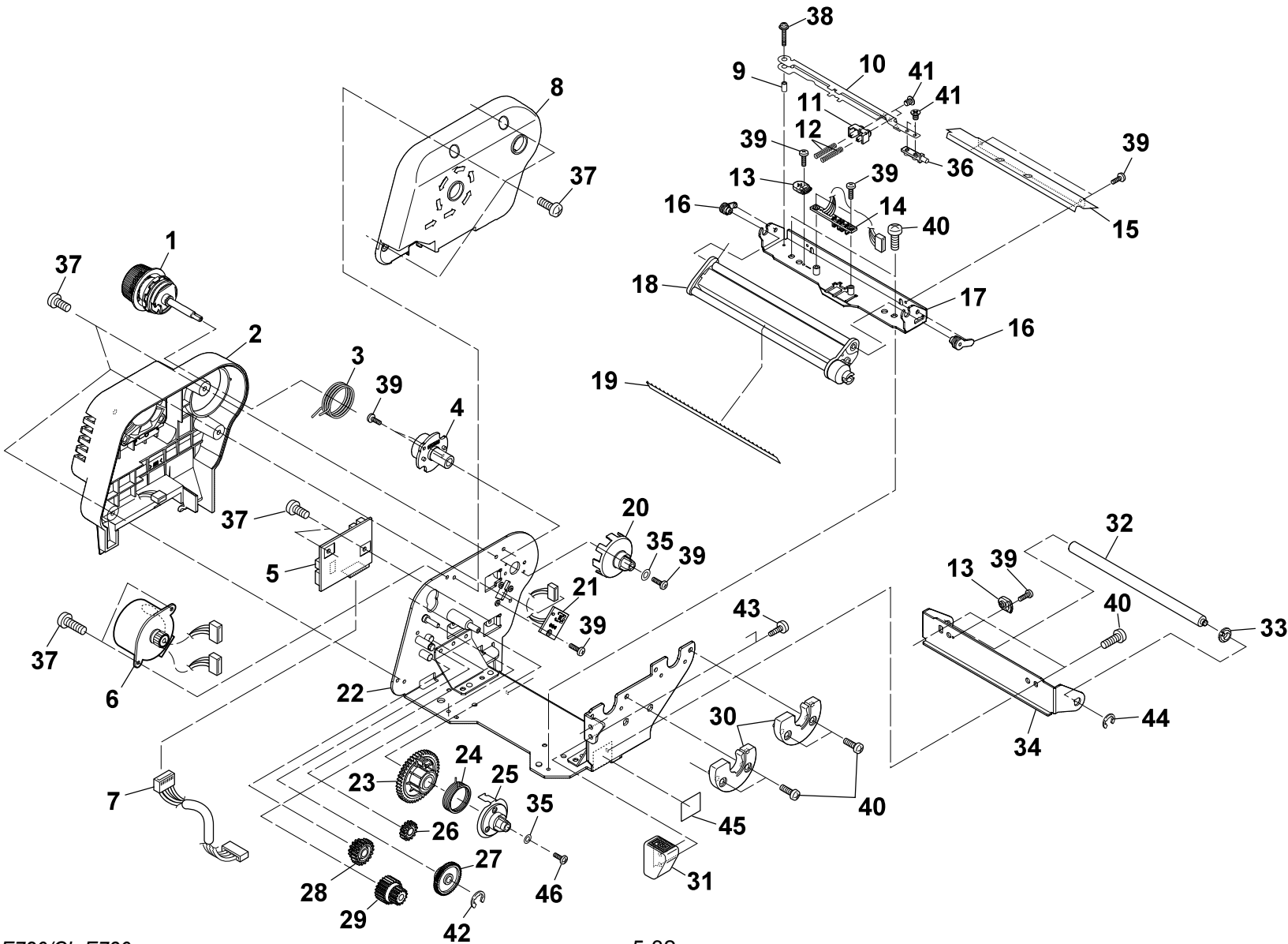
DRAWING NO. 8 Unit Ribbon (Rev. 0)
